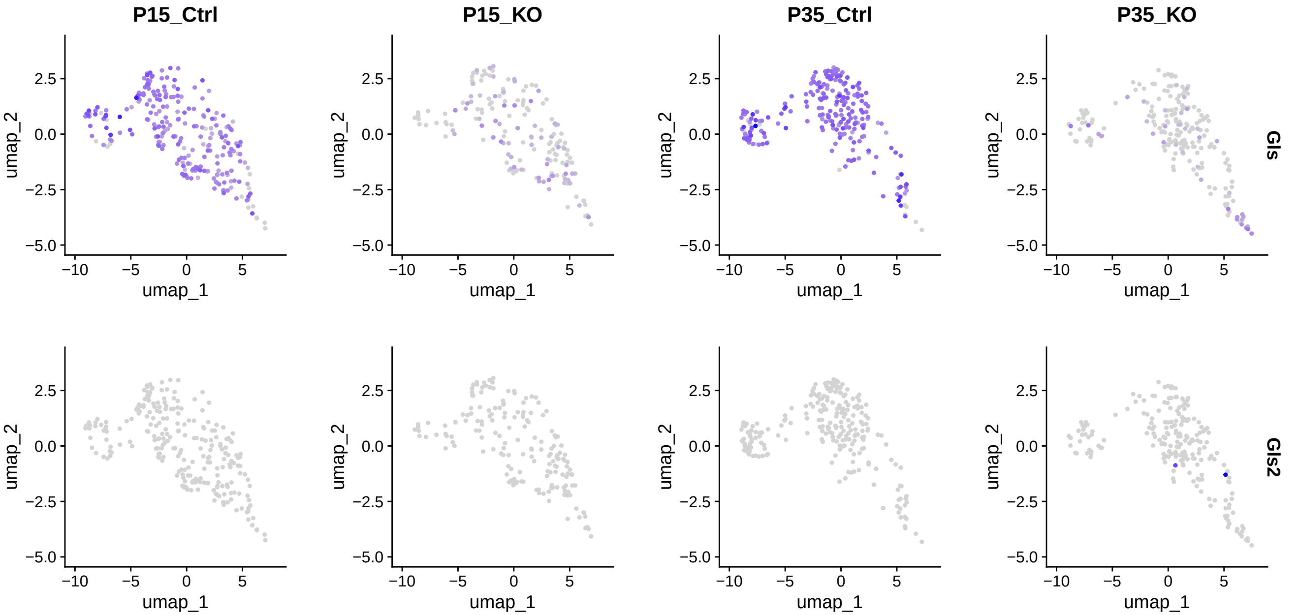
Reclustered cones: GlIs/GIs2 on UMAP by age and condition
