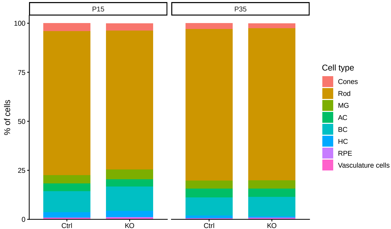
Cell type composition by age and condition
