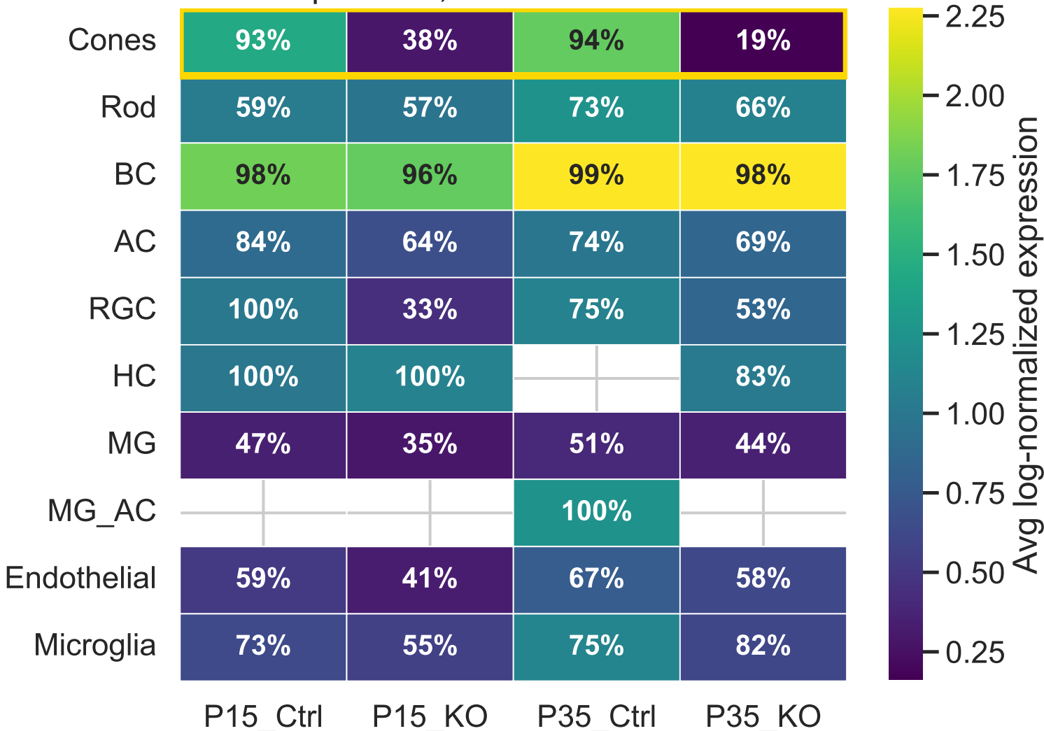
Gls expression; labels show % detected
