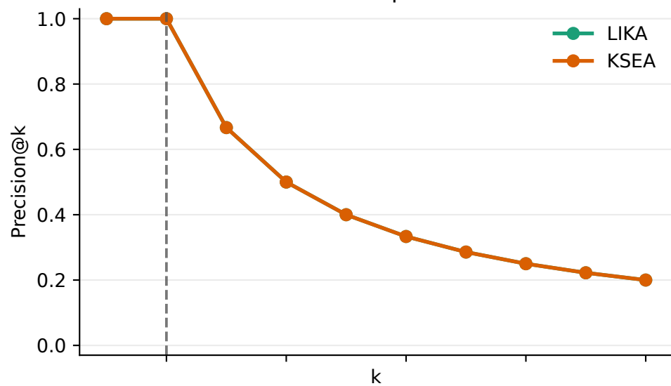
Simulation Experiment 2
