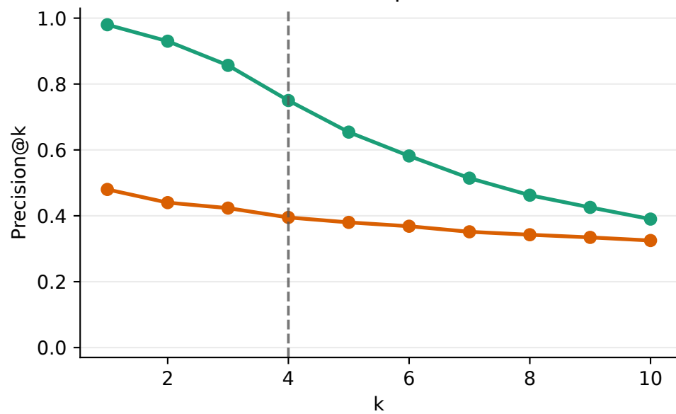
Simulation Experiment 3
