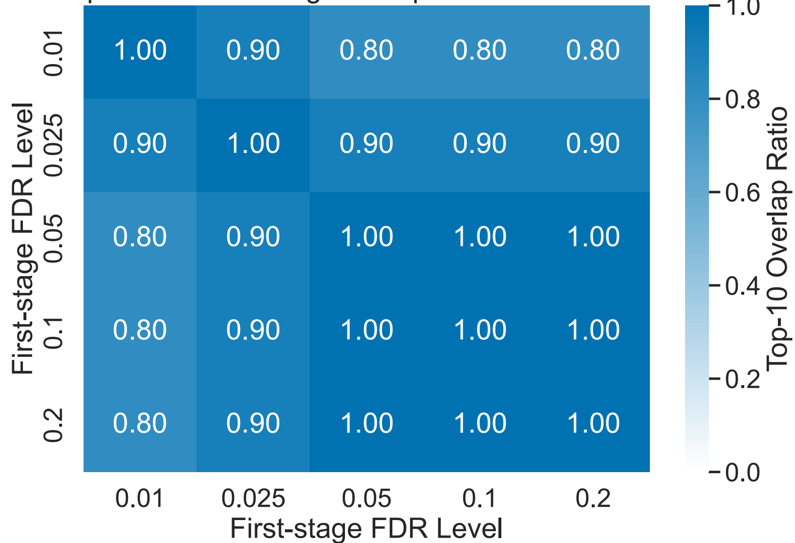
Top-10 LIKA Ranking Overlap Across FDR Levels
