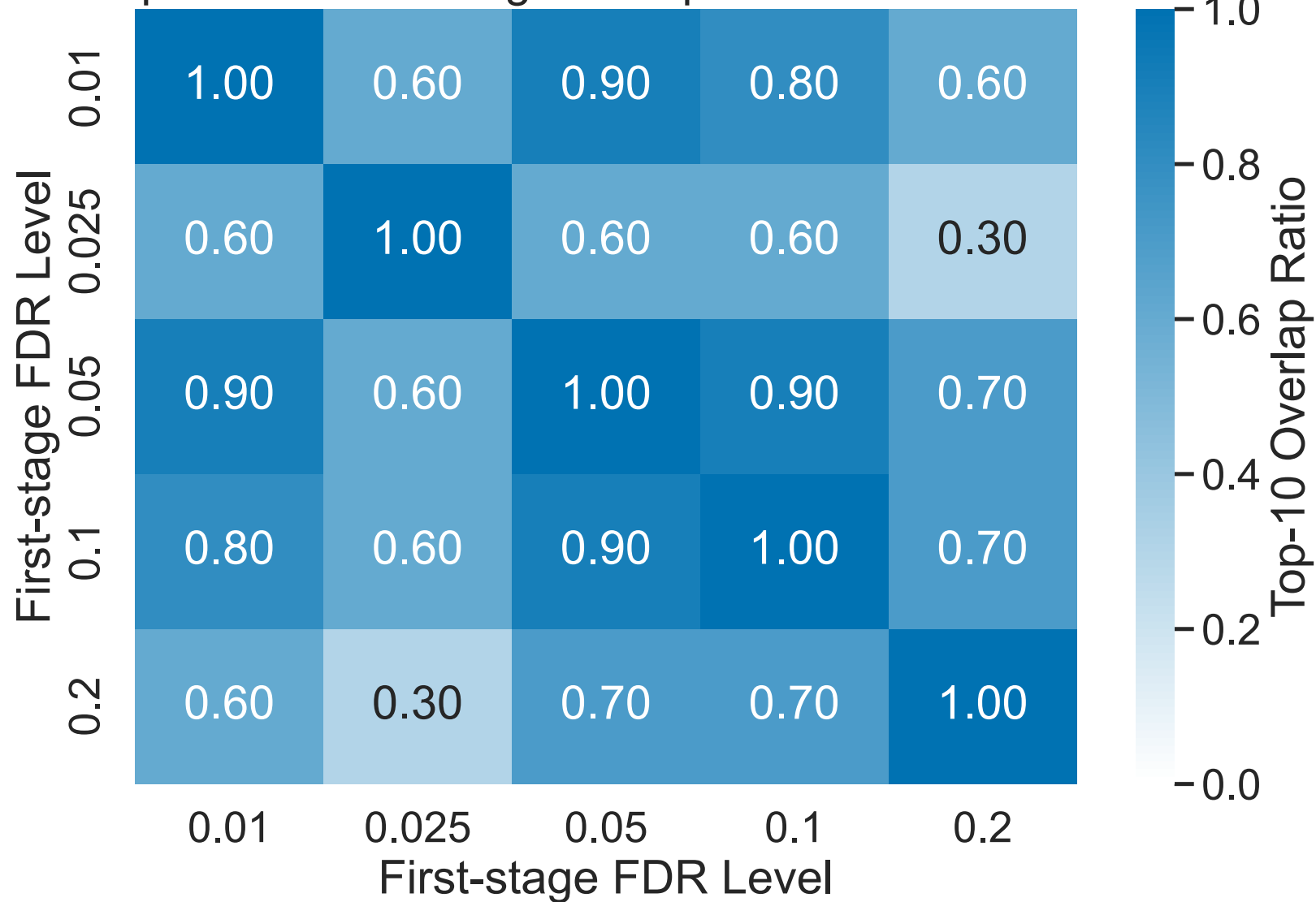
Top-10 LIKA Ranking Overlap Across FDR Levels
