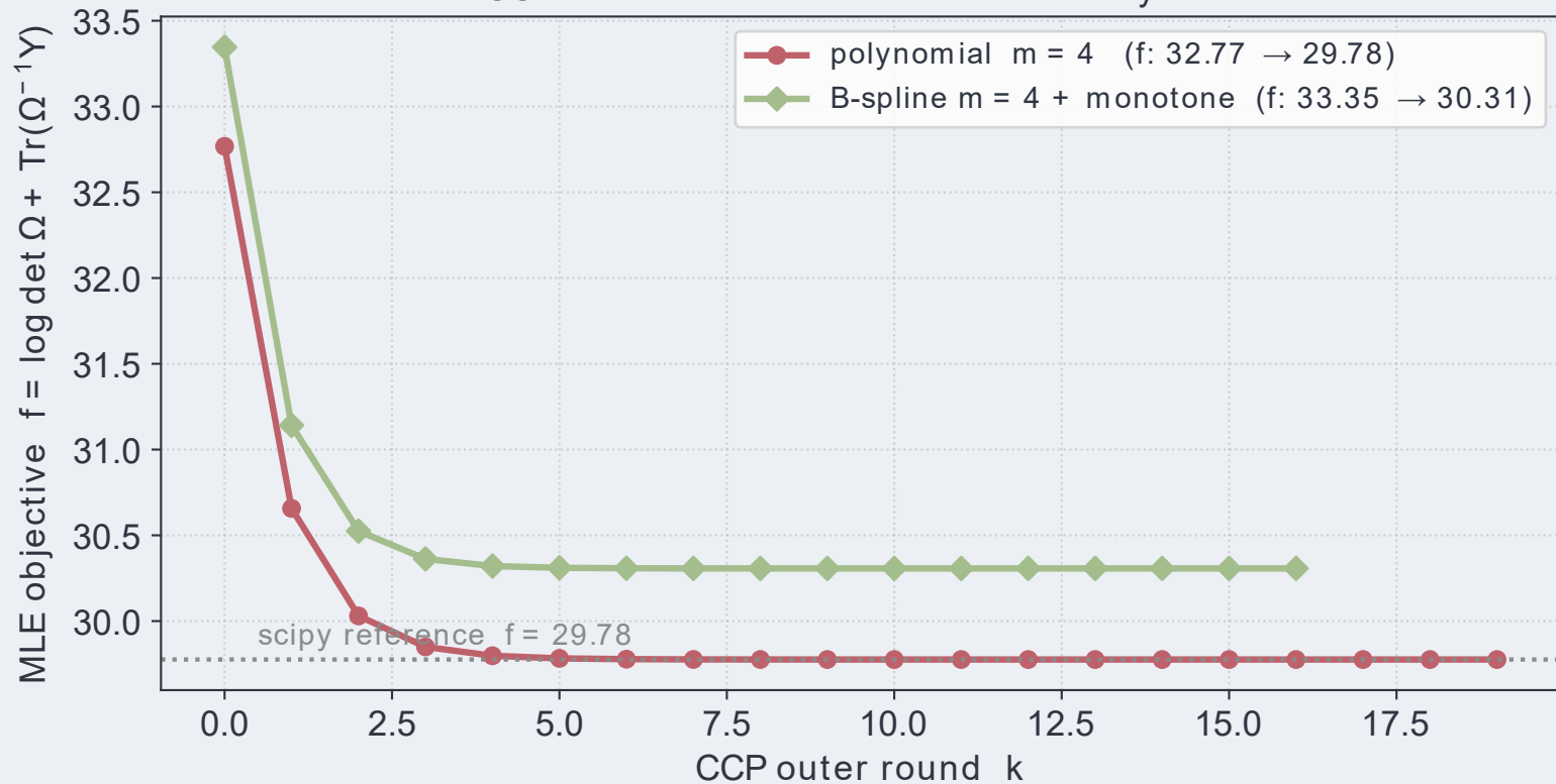
CCP: monotone decrease to the free family MLE
