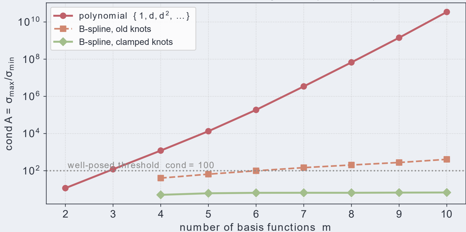
Condition number of the design matrix (n = 20 sites)
