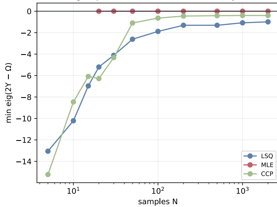
2Y margin: pinned at 0 \Rightarrow constraint always active
