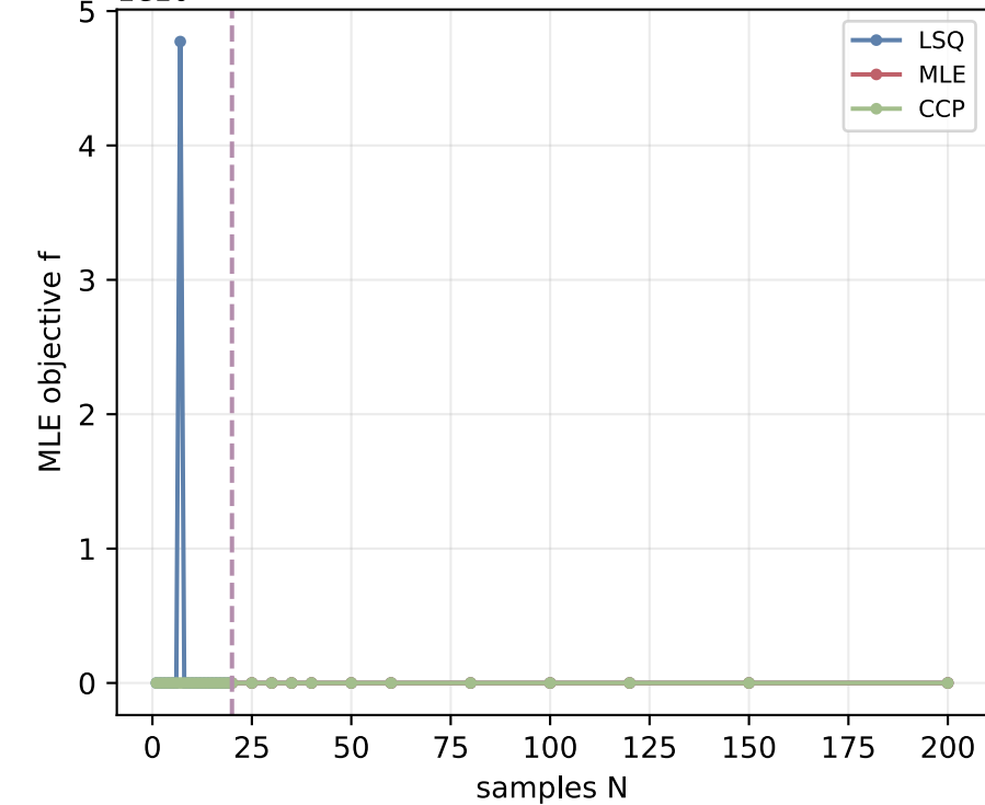
MLE objective
