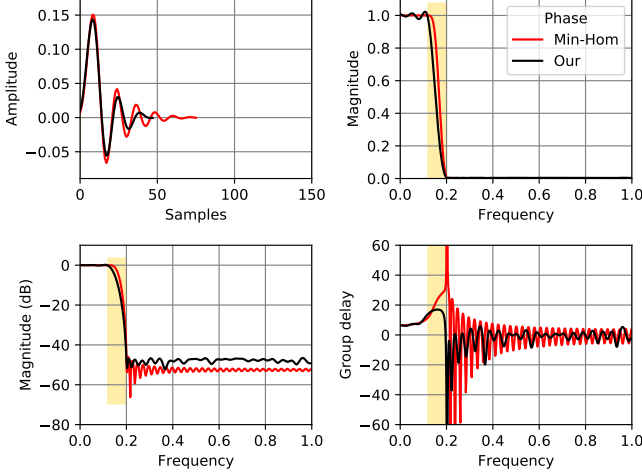
Figure 3: Magnitude response of a lowpass design.
