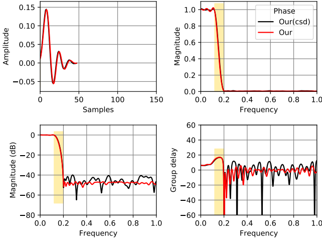
Figure 4: Magnitude response after CSD quantization.
