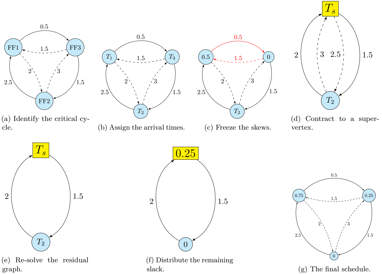
Figure 9: The iterative EVEN (minimum-balancing) process on a small timing constraint graph: identify the most critical cycle, distribute its slack evenly, freeze the arrival times, contract the cycle to a super-vertex, and repeat until a single vertex remains (illustration from the lecture).
