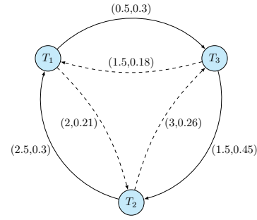
Figure 8: A statistical timing constraint graph: after SSTA each edge carries a pair (\mu, \sigma) —mean and standard deviation—instead of a single deterministic weight (illustration from the lecture).
