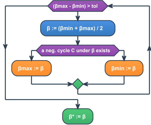
Figure 16: Lawler’s binary-search algorithm: bisect the bracket [\beta_{\min}, \beta_{\max}] and test the timing constraint graph for a negative cycle; the upper or lower bound is updated until the tolerance is met.
