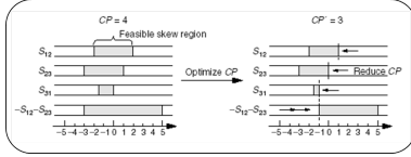
Figure 7: After period minimization, many skews sit on the boundary of their feasible skew regions; the narrow margins that remain are what process variations consume, which motivates yield-driven scheduling (illustration from the lecture).
