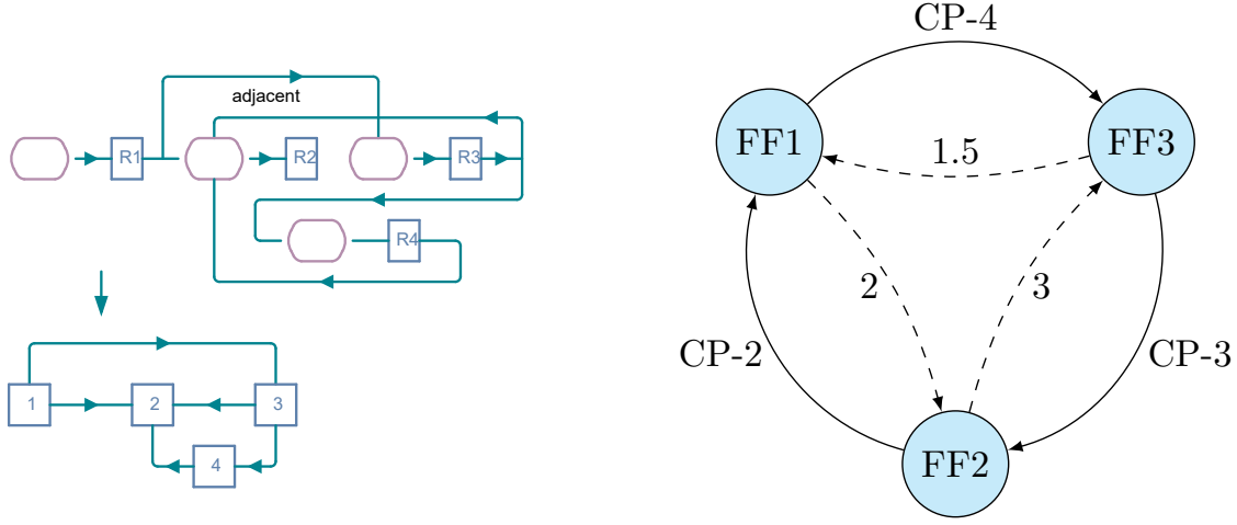
Figure 3: A circuit and its timing constraint graph. Solid arcs are setup constraints ( s -edges); dashed arcs are hold constraints ( h -edges). The weights are T_{CP} - 4 and 1.5, etc.
