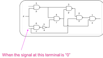
Figure 10: A false path: although a structural path exists, no input pattern sensitizes it, so it carries no signal and must be excluded from the timing constraints (illustration from the lecture).
