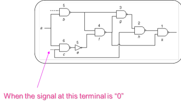
Figure 10: A false path: although a structural path exists, no input pattern sensitizes it, so it carries no signal and must be excluded from the timing constraints.
