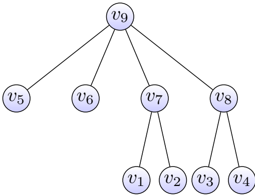
Figure 12: The contraction tree: each super-vertex merges a critical cycle, and the final arrival time of a register is the sum of the frozen arrival times along its root path—for example, T_1^{\text{final}} = T_1 + T_7 + T_9 .
