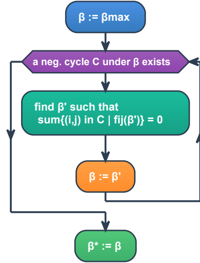
Figure 17: Howard’s policy-iteration algorithm: a cycle of the current policy yields an improved \beta , after which a new policy is computed from the parameterized shortest paths.
