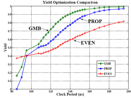
Figure 13: A comparison of the yield-driven scheduling methods on a common example.
