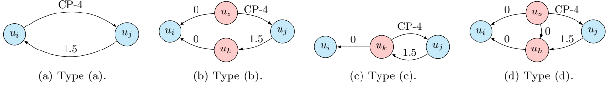
Figure 6: The four structural configurations for delay insertion. Type (a): no feasible insertion; (b): p_s, p_h independent; (c): p_s = p_h ; (d): p_s \geq p_h .
