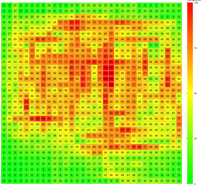
Figure 4: Combined congestion map (element-wise maximum of the x- and y-direction maps) for the 32x32 placement.
