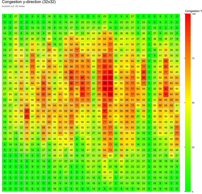
Figure 3: Congestion in the y-direction for the same placement, normalized to the busiest vertical cut.
