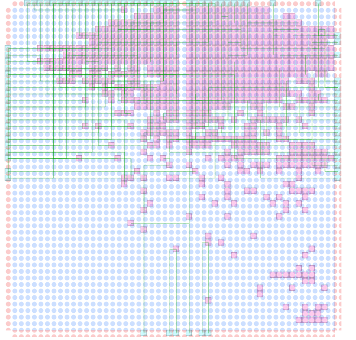
Figure 7: Routed placement on the 50x50 grid: orthogonal routing trees replace the straight proxy connections.
