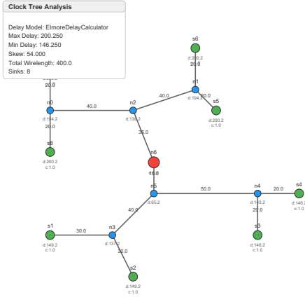
Figure 10: The same topology under the Elmore model: realistic RC delays with the prescribed skew preserved.
