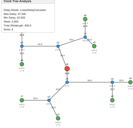
Figure 9: A prescribed-skew clock tree under the linear delay model; the panel reports maximum/minimum delay, skew and total wirelength.
