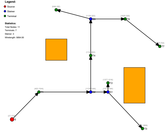
Figure 6: Global routing with Steiner-point insertion and rectangular keepouts (orange): the tree avoids the obstacles and shares segments between terminals.
