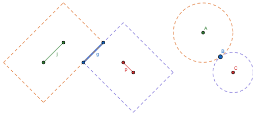
Figure 4: The L_1 merging-segment operations: intersecting two enlarged Manhattan arcs (left) is the analogue of intersecting two circles (right) in a Euclidean Voronoi construction.
