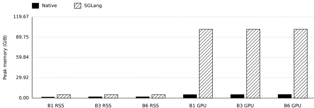
Figure 4. Peak process RSS and GPU-visible unified memory. Native is solid; SGLang is diagonal-hatched.
