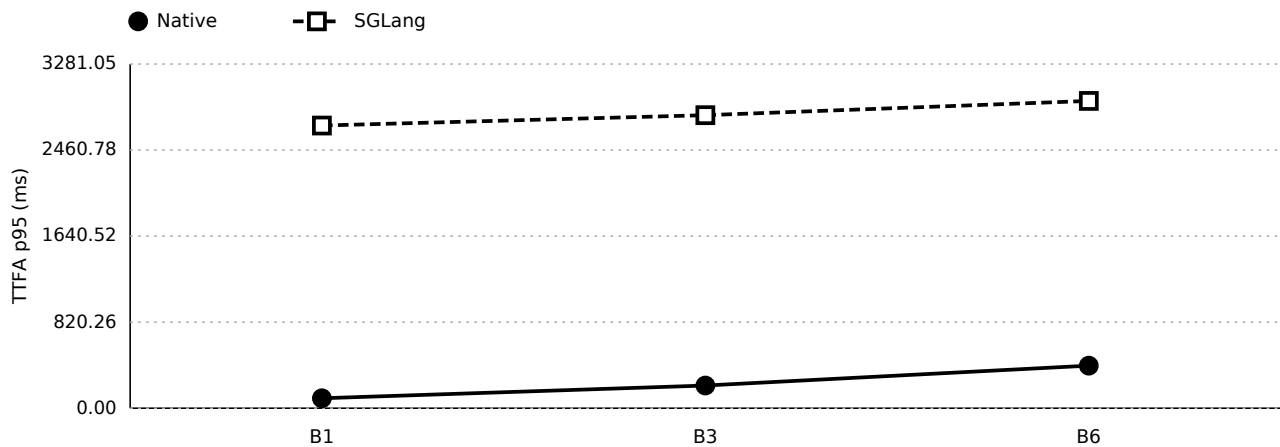
Figure 1. TTFA p95 by concurrency. Native uses a solid line and circle markers; SGLang uses a dashed line and square markers.
