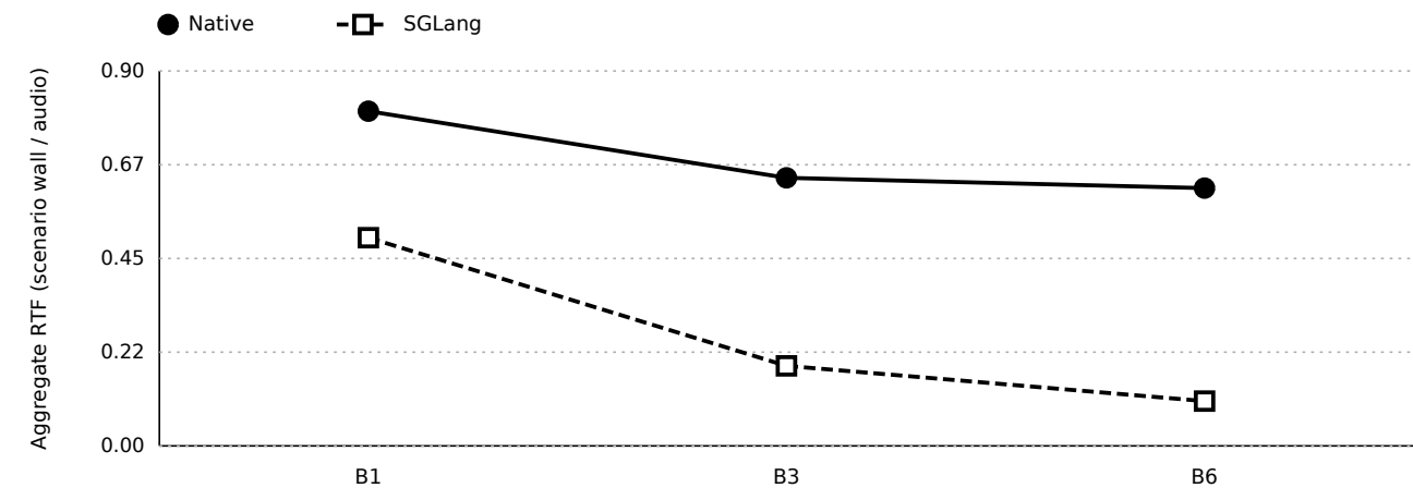
Figure 2. Scenario aggregate RTF by concurrency. Values below 1.0 mean the measured scenario produced audio faster than real time.
