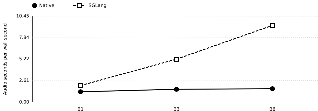
Figure 3. Aggregate audio throughput over each measured profile run.
