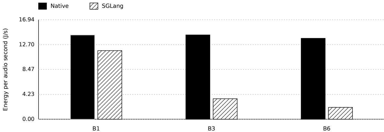
Figure 5. Request energy normalized by successful emitted audio duration.
