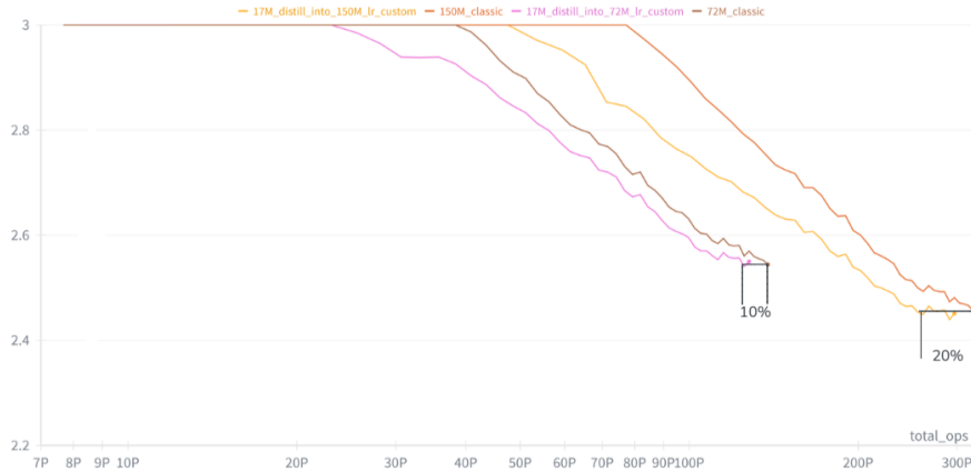
Figure 3: Validation loss vs compute (including teacher-training compute) showing \sim 10\% compute savings for 17M \rightarrow 72M and \sim 20\% savings for 17M \rightarrow 150M.
