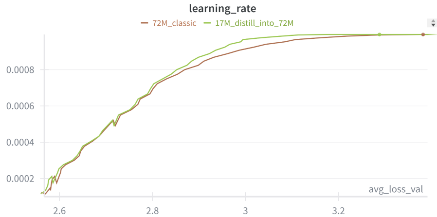
Figure 7: Learning rate vs validation loss for 17M→72M bootstrapped distillation vs classical training. Parameterizing training by validation loss reveals a tight link between learning rate and achievable loss: once KD ends and the learning-rate profiles align, trajectories become near-identical.
