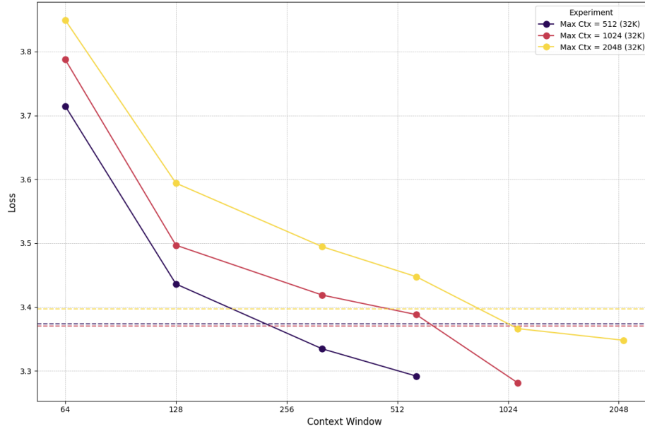
Figure 5: Context-length sweep for the 5M-parameter model (batch size 32k tokens). Compared to the 1M case, this larger model benefits from a longer maximum context; in this sweep, 1024 performs best while 2048 offers no consistent improvement.
