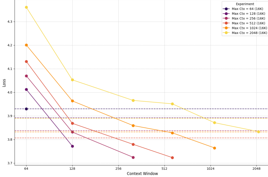
Figure 4: Context-length sweep for the 1M-parameter model (batch size 16k tokens). A maximum context length around 512 yields the best losses in this regime, while very long contexts ( \geq 1024 ) degrade performance.
