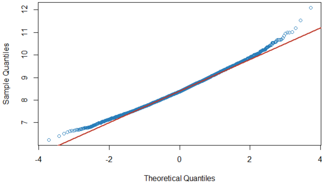
Q-Q Plot - Log-transformisani prihod
