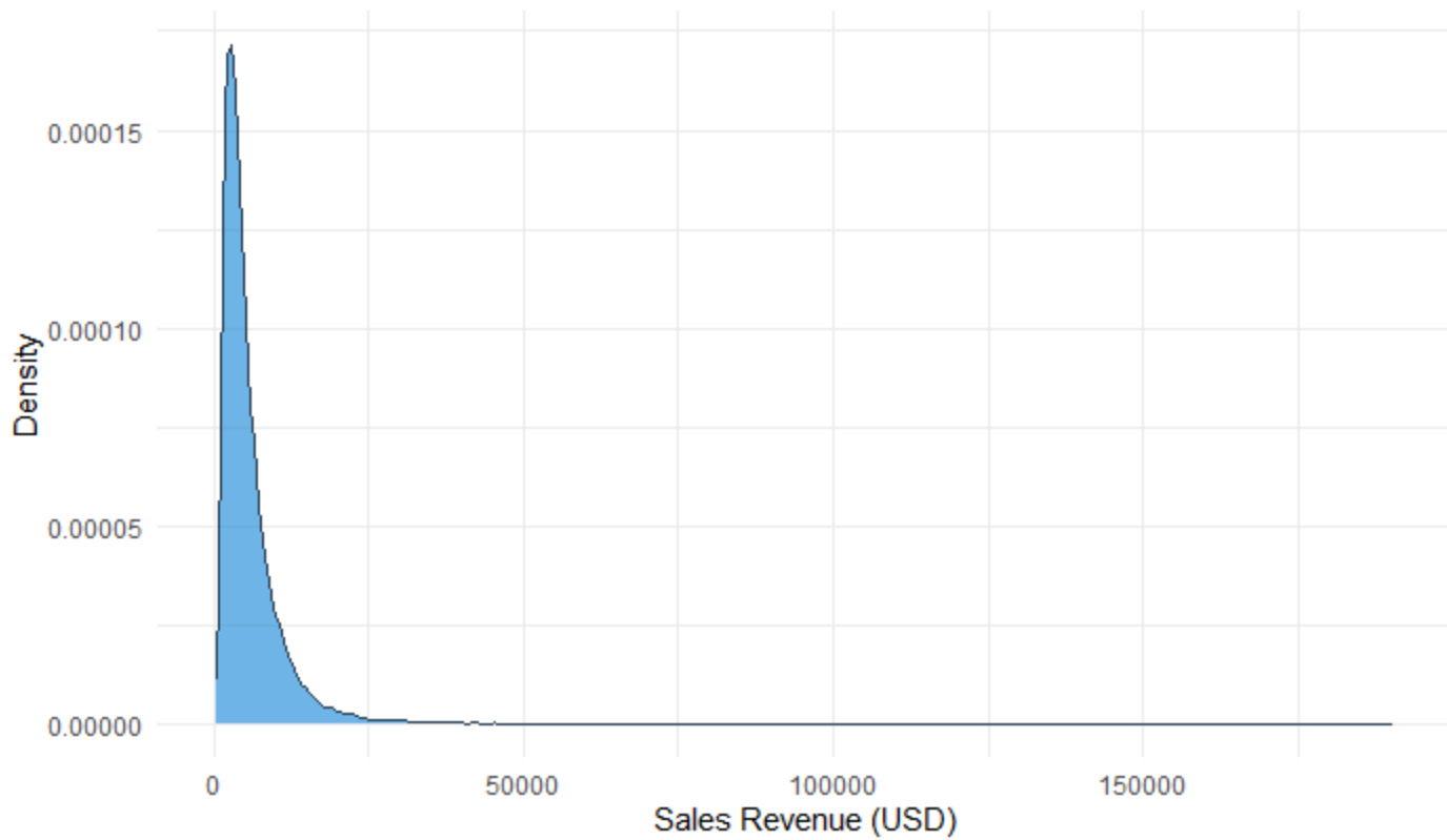
Density Plot: Sales Revenue
