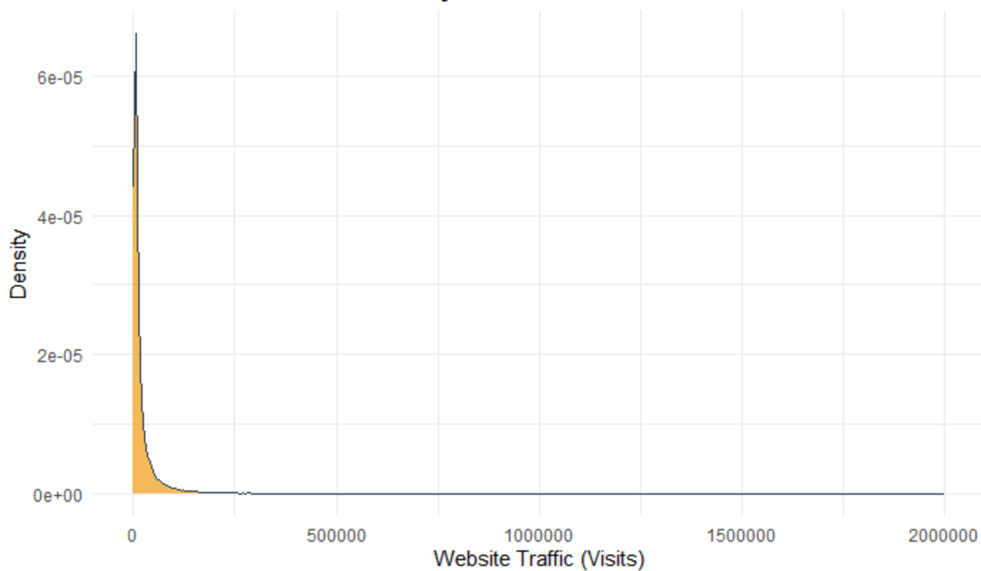
Density Plot: Website Traffic
