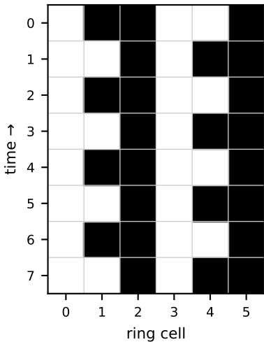
ring rotor on \mathbb{Z}/6 : hop 3/step
