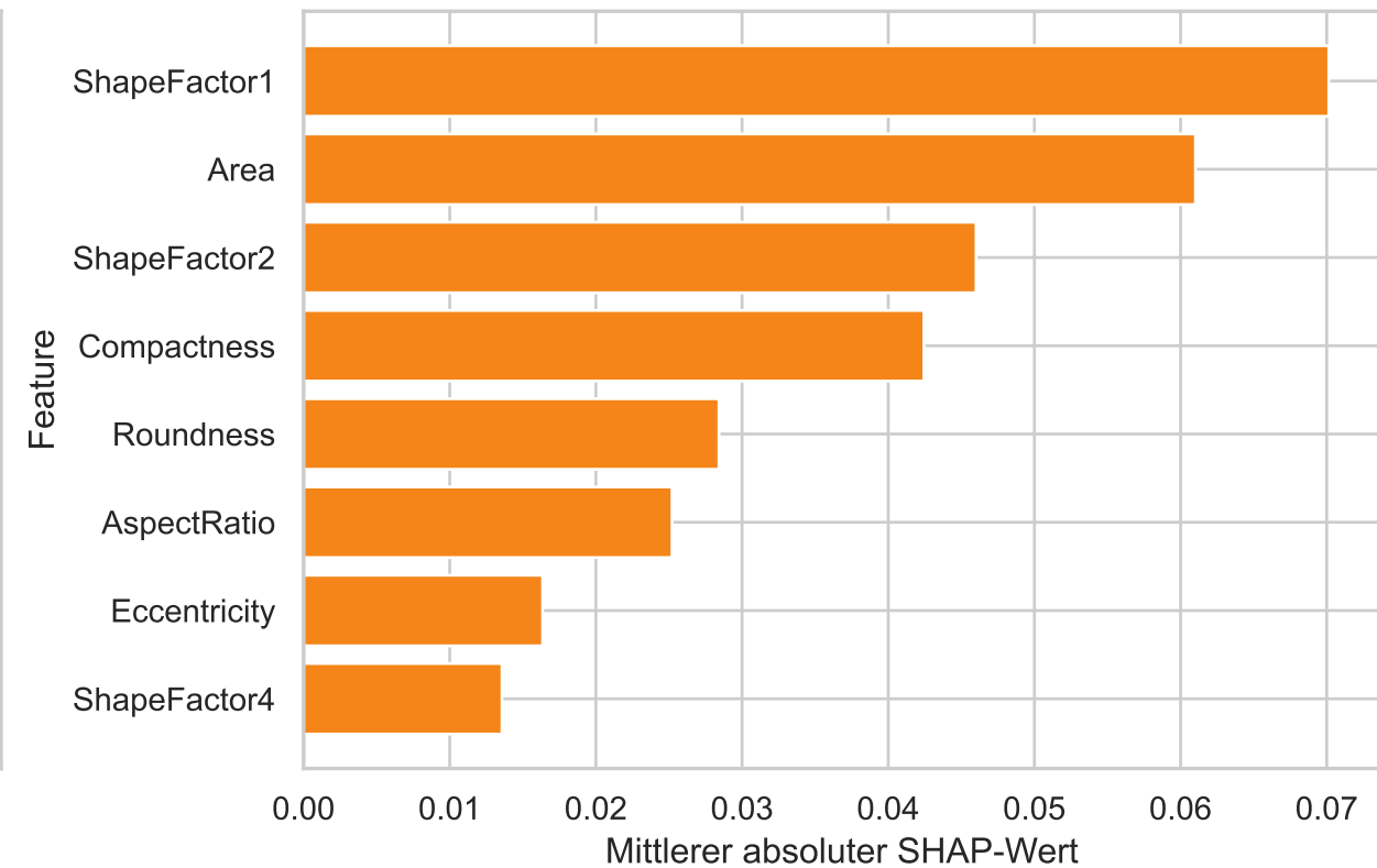
MLP Neural Network
