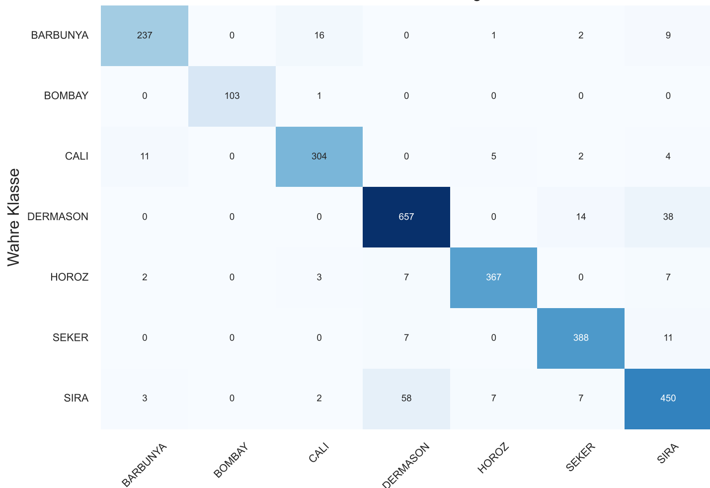
HistGradientBoosting
