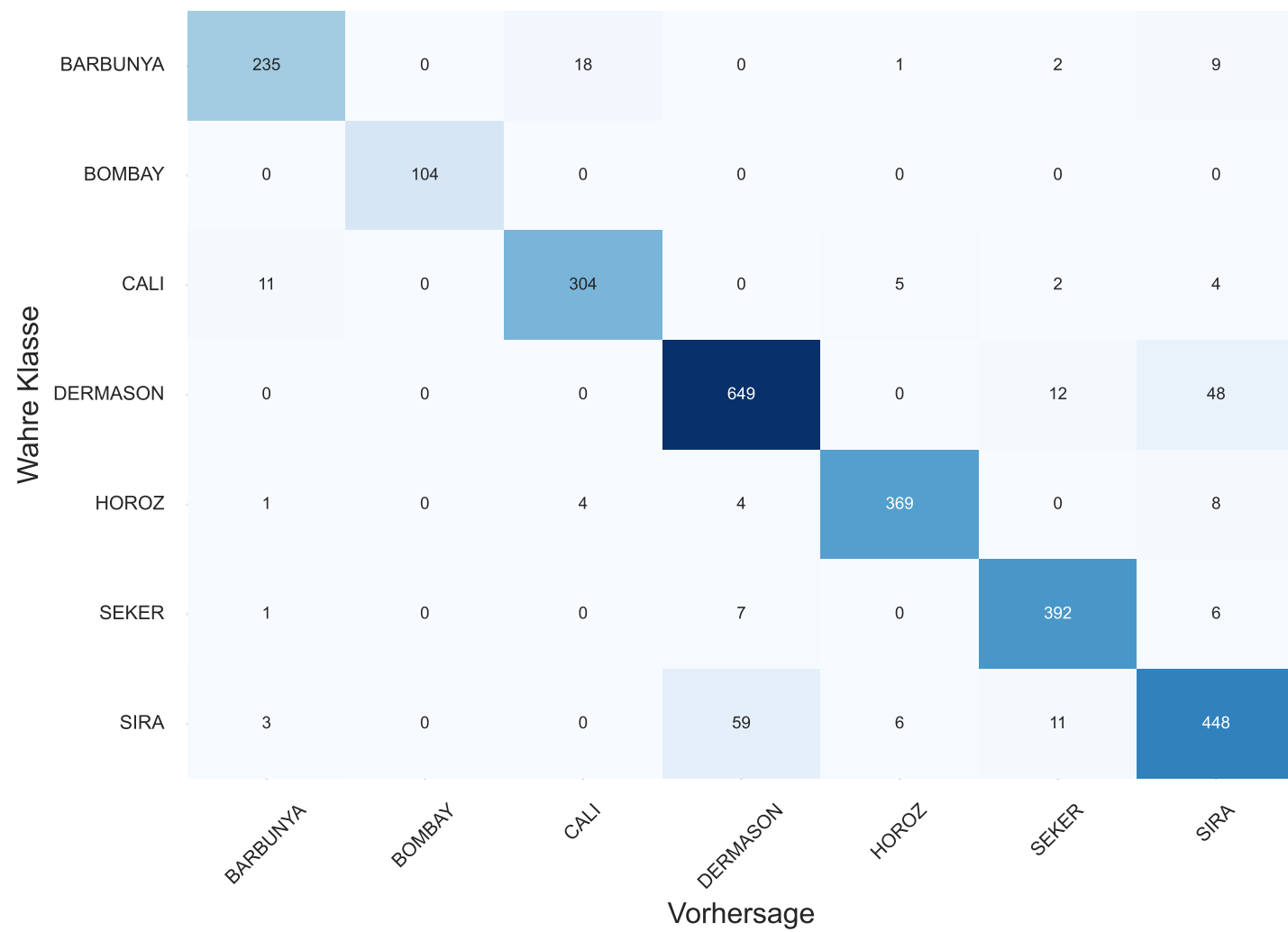
Random Forest
