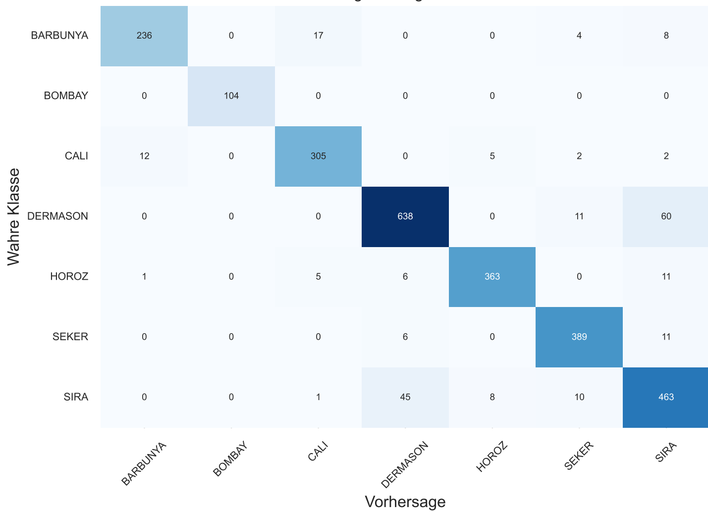
Logistic Regression
