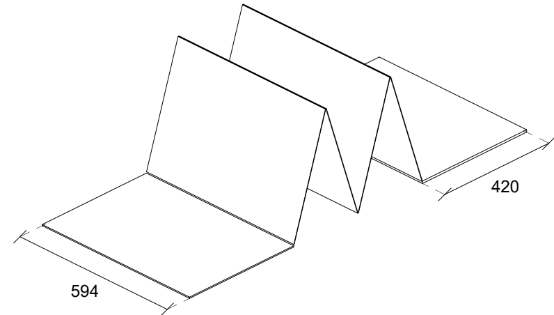
Accordion 24 sheets A2 joined along the long edge, folded 420 x 594, 10.08 m unfolded, drawn 1:15
