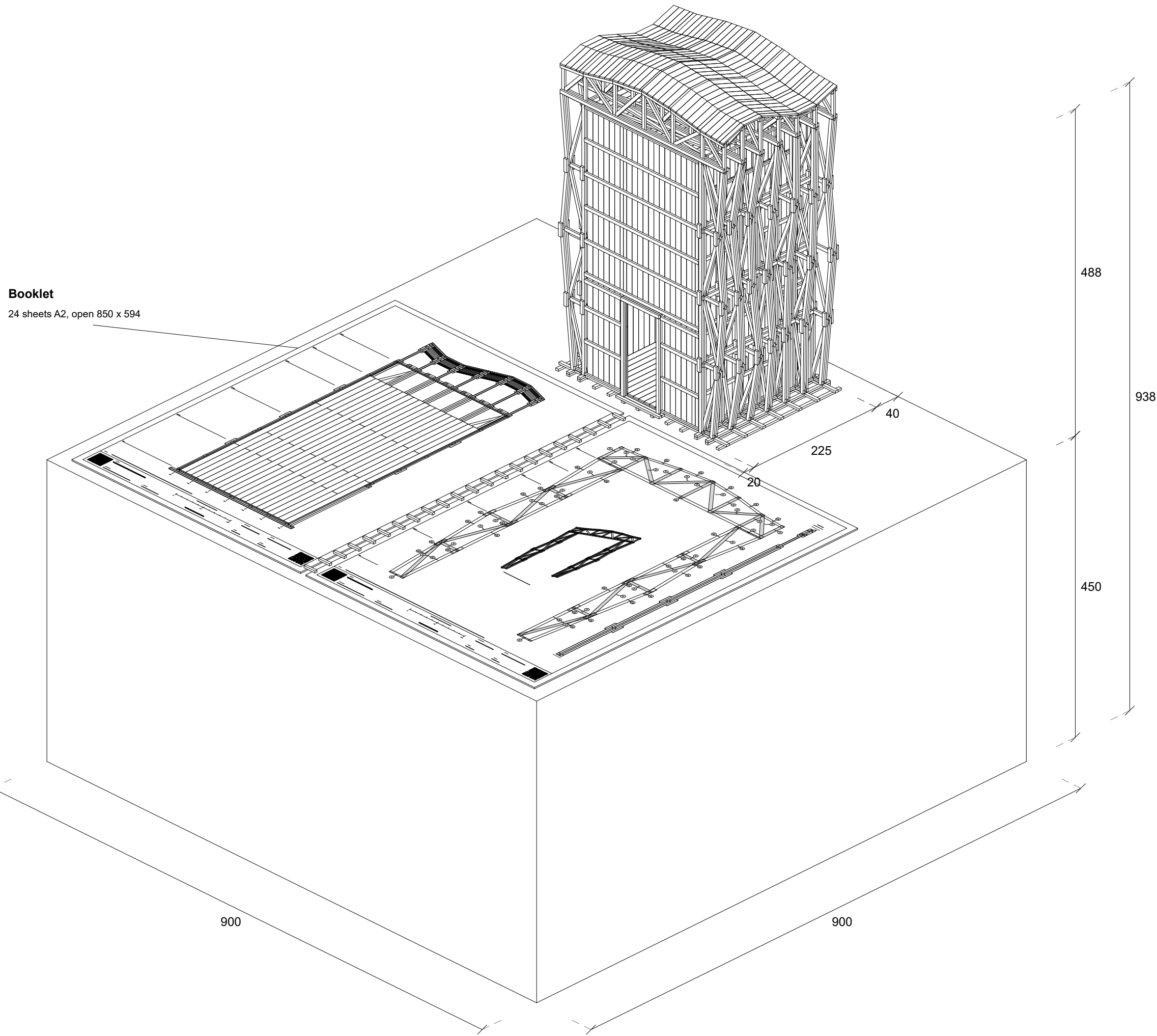
Axonometric 1:5, seen from the door side, with the booklet
