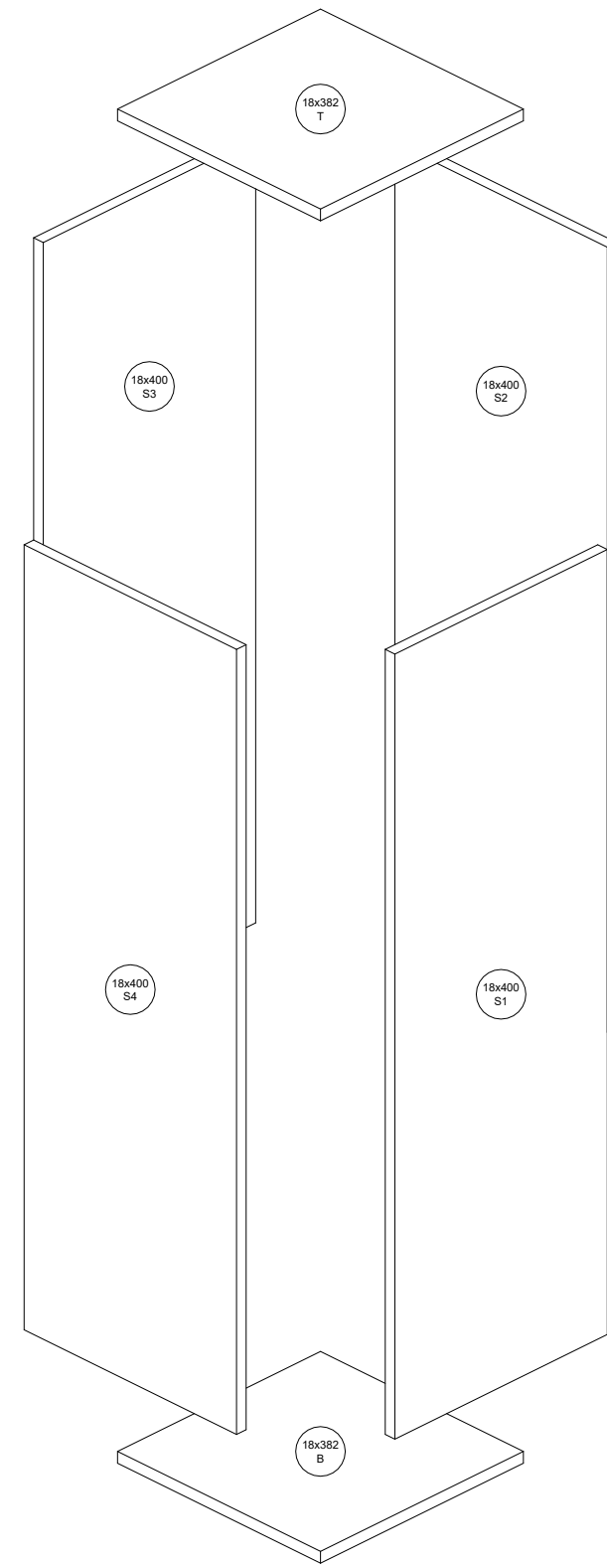
Pedestal exploded, 1:10
