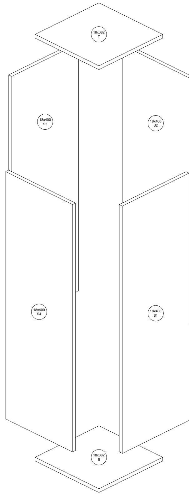
Pedestal exploded, 1:10
