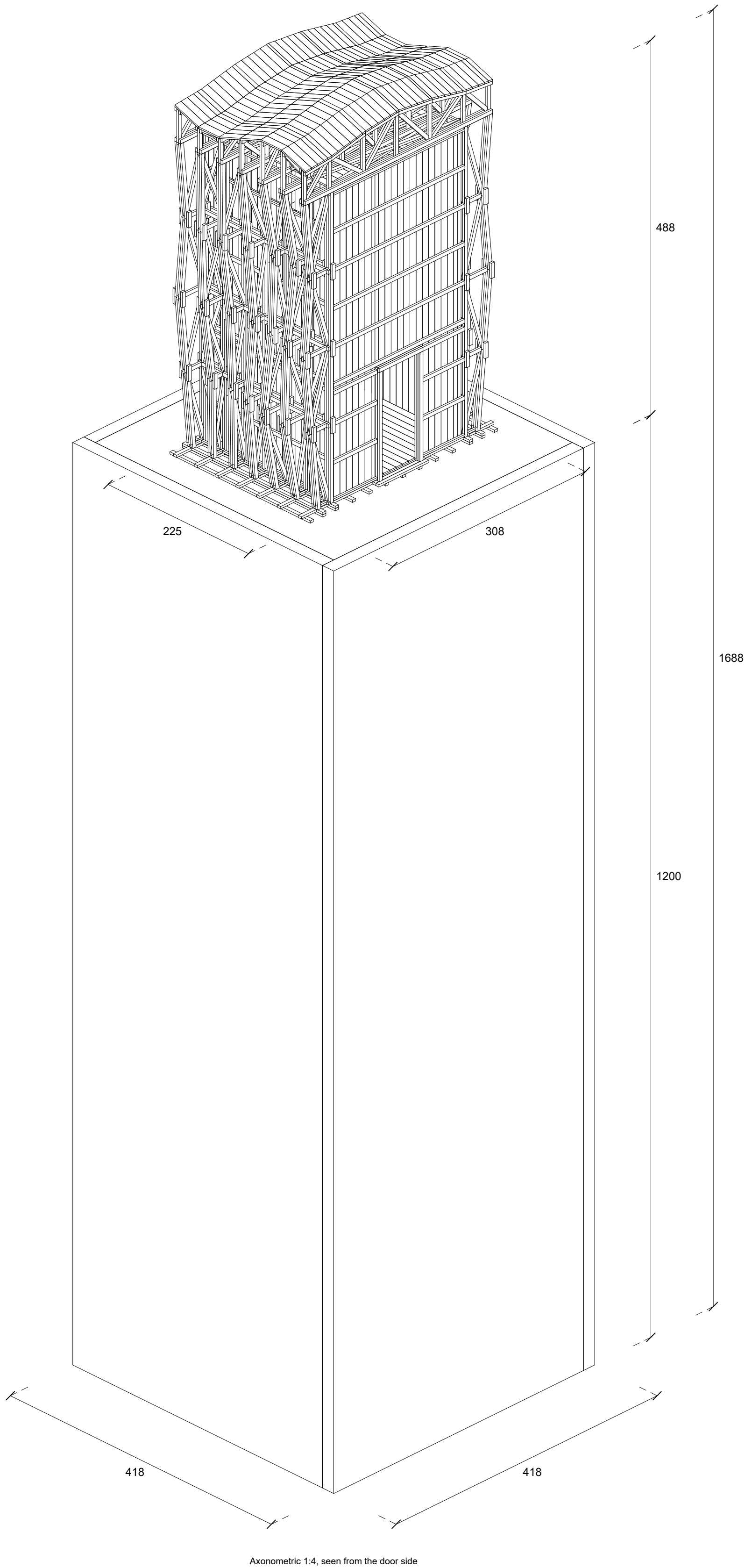
Axonometric 1:4, seen from the door side
