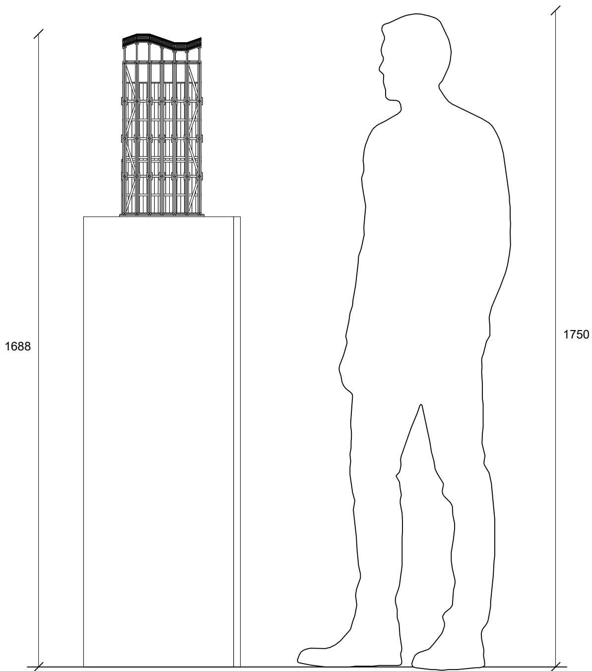
Side view 1:10 with a visitor 1.75 m tall
