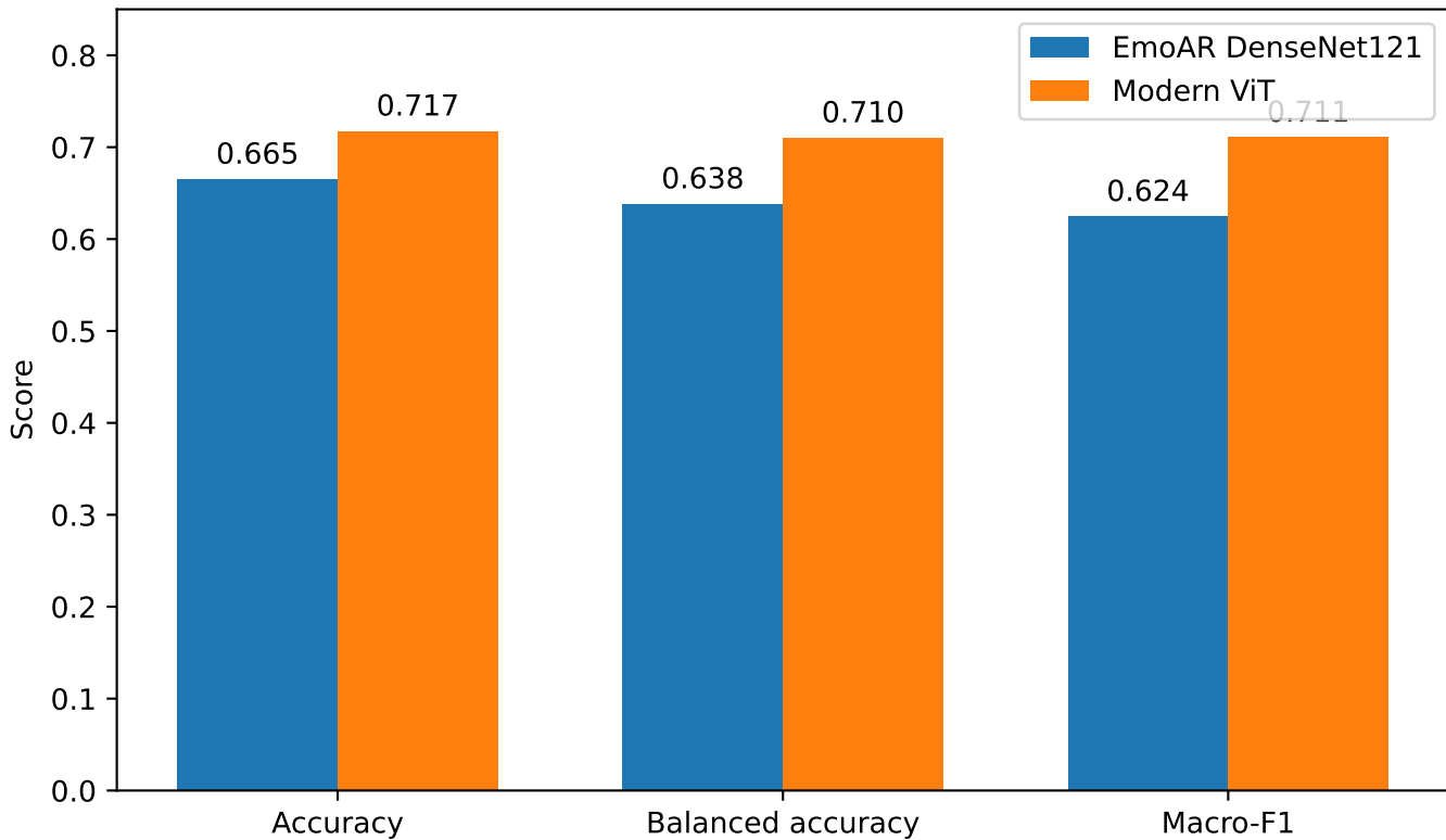
FER2013 privateTest classification performance
