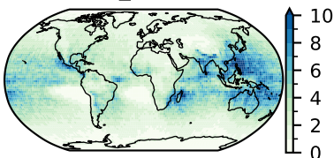
CanESM5 (25)
