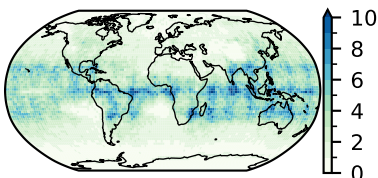
GFDL-CM3 (20)
