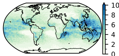
CanESM2 (50)
