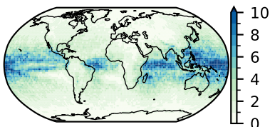
GFDL-SPEAR-MED (30)
