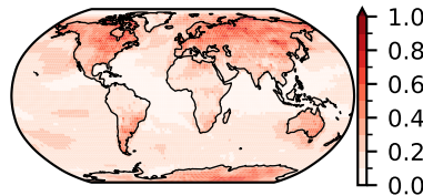
CanESM5 (25)
