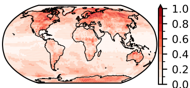
UKESM1-0-LL (16)
