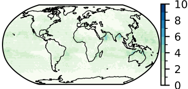
UKESM1-0-LL (16)
