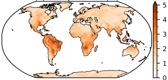
(f) WSDI StdDev (days)
