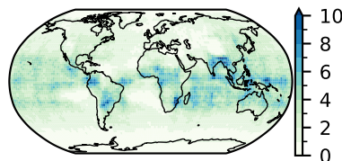
EC-Earth3 (18)
