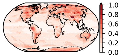
EC-Earth3 (18)
