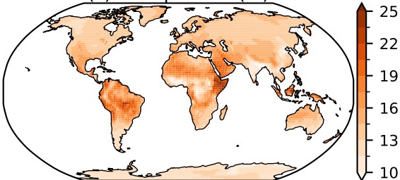
(e) WSDI mean (days)
