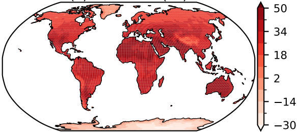
(c) TX90p mean (%)
