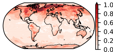
IPSL-CM6A-LR (33)
