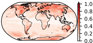
GFDL-SPEAR-MED (30)
