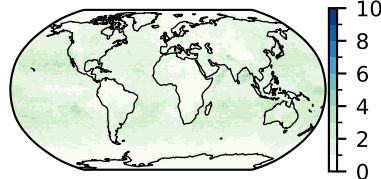
MPI-ESM1-2-LR (50)
