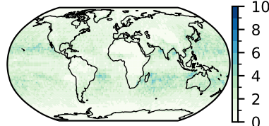
IPSL-CM6A-LR (33)
