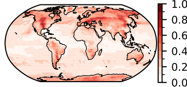
MPI-ESM1-2-LR (50)
