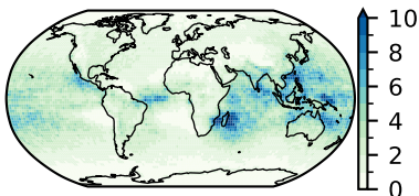
CSIRO-Mk3-6-0 (30)
