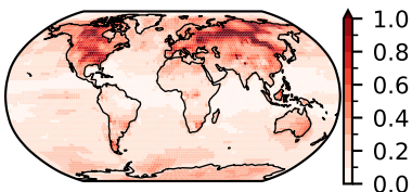
GFDL-ESM2M (30)
