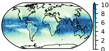
MIROC6 (50)
