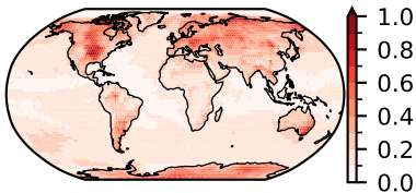
CanESM2 (50)
