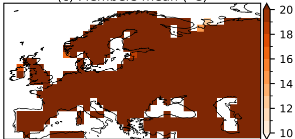
(c) Members mean ( ^{\circ}\text{C} )
