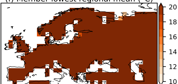
(f) Member lowest regional mean ( ^{\circ}\text{C} )
