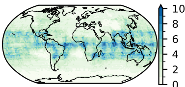
GFDL-CM3 (20)
