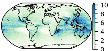
CanESM5 (25)
