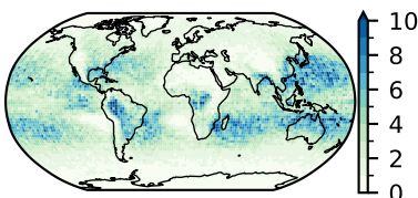
UKESM1-0-LL (16)
