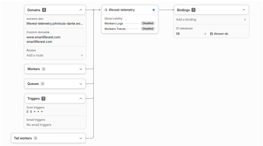
Figure 2: Cloudflare workers and bindings for deployment.
