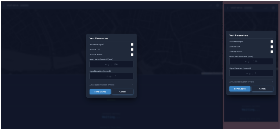
Figure 6: UI for Dashboard settings modal in desktop and phone formats.
