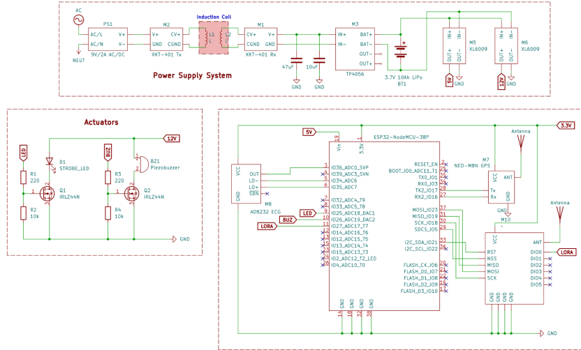
Figure 10: Schematic diagram of the device.
