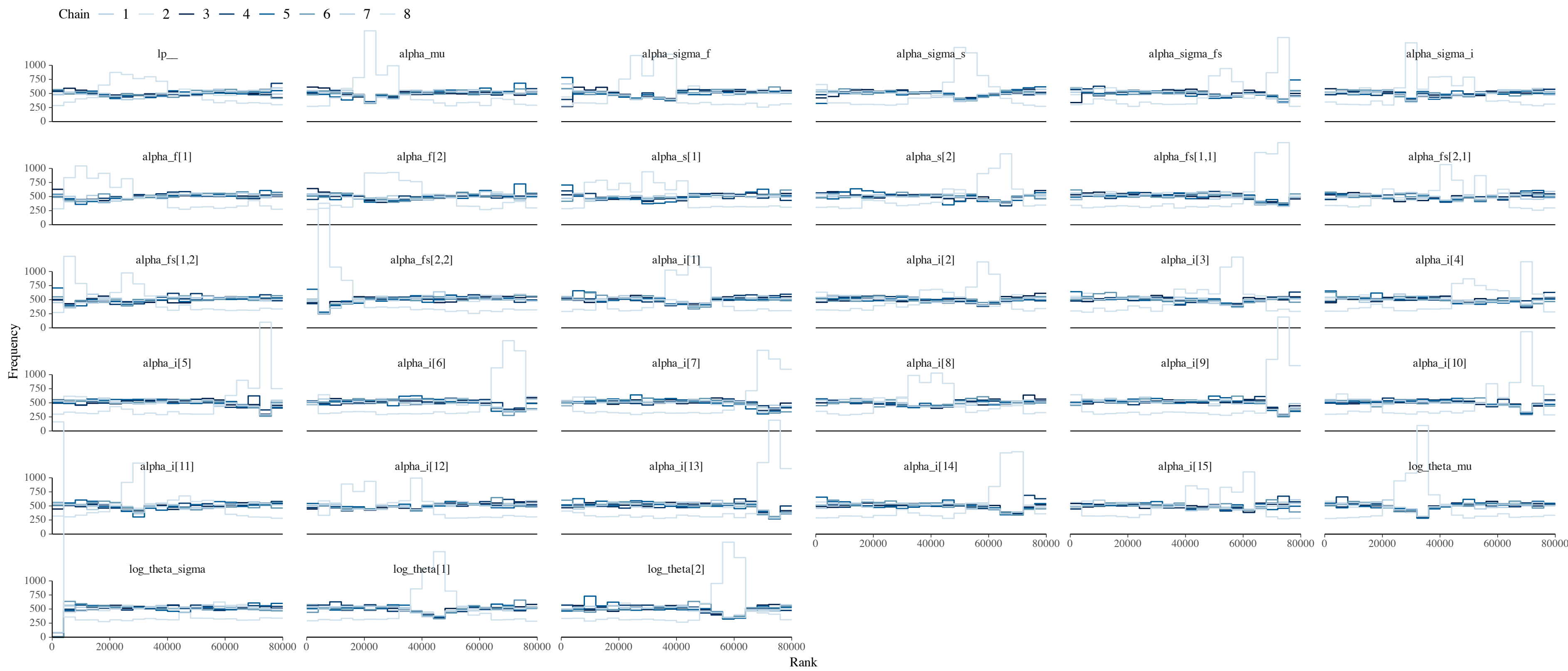
Non-centred model
