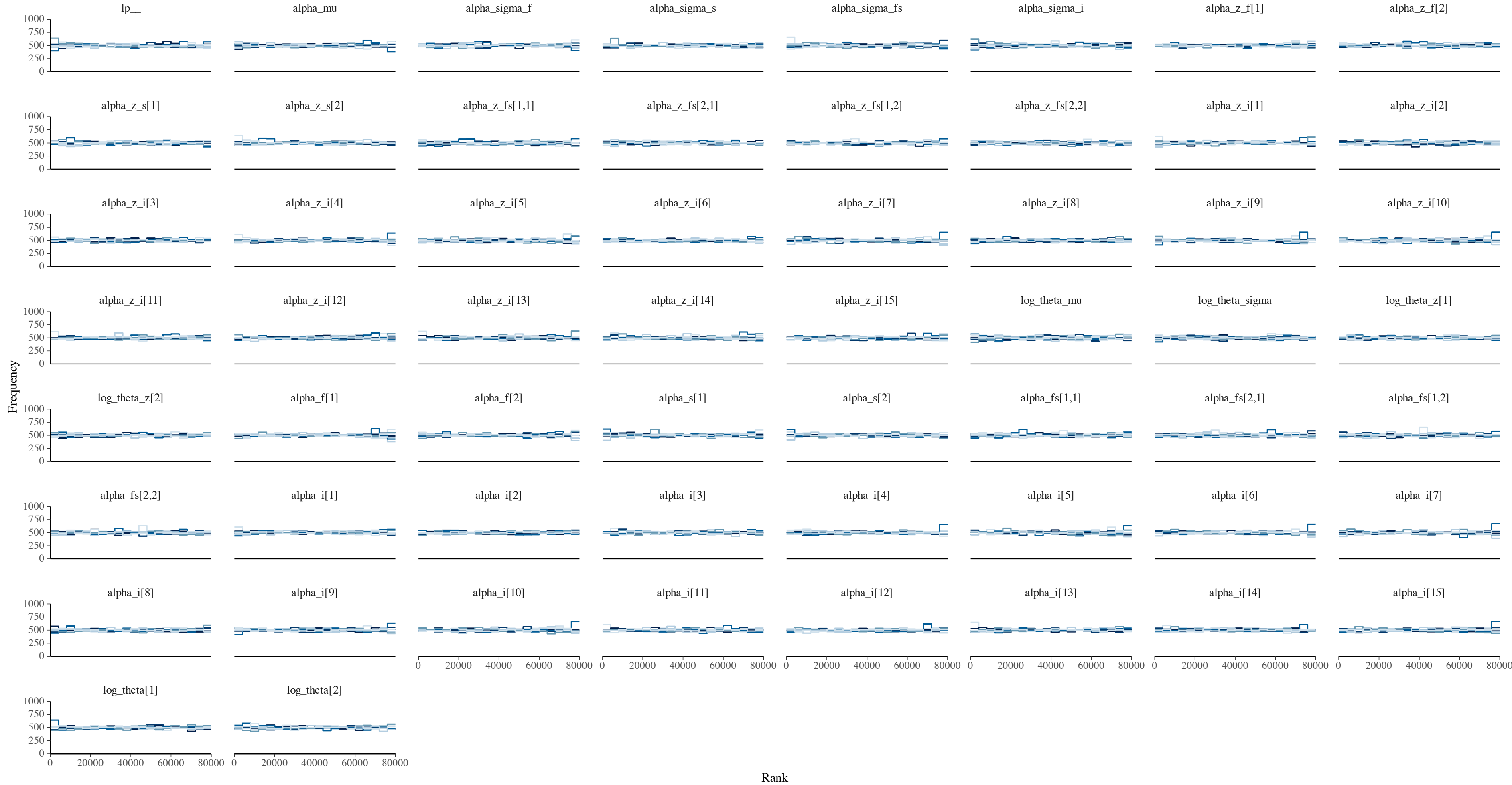
Non-centred model
