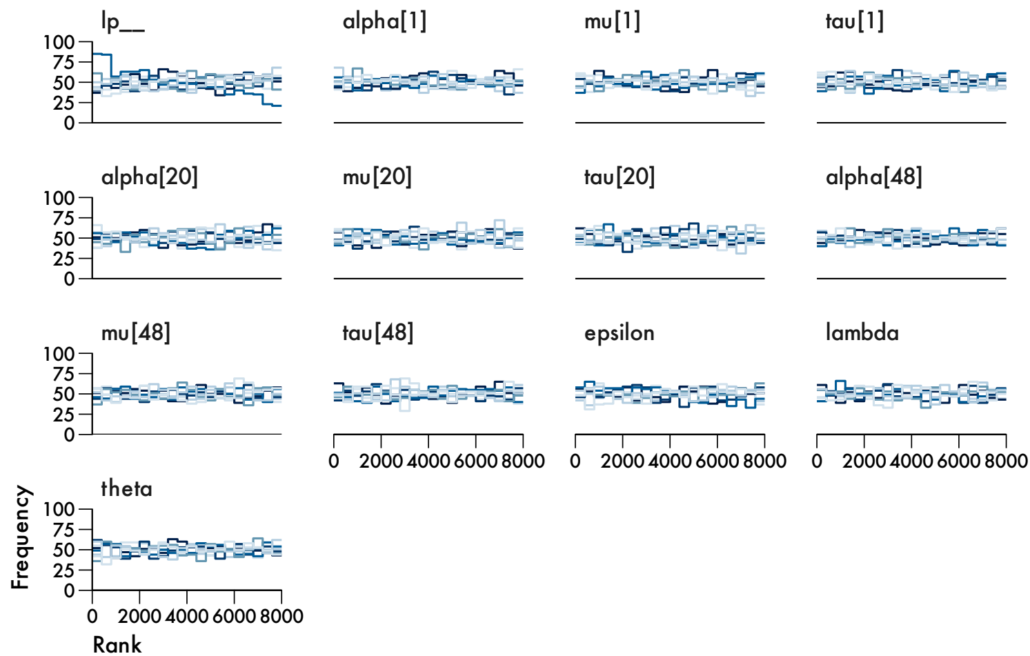
Beta prime likelihood with heterogenous variance
