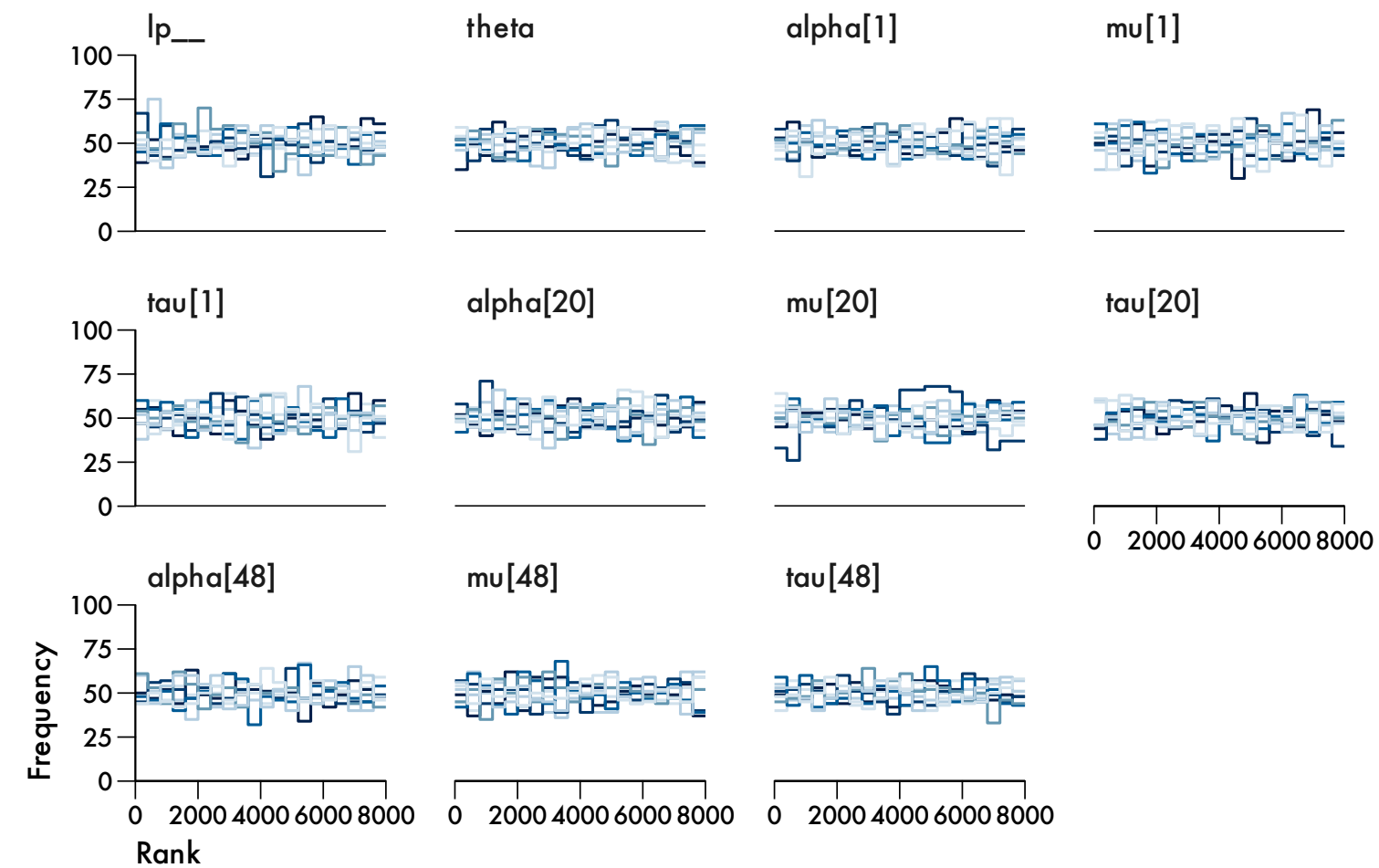
Beta prime likelihood with homogenous variance
