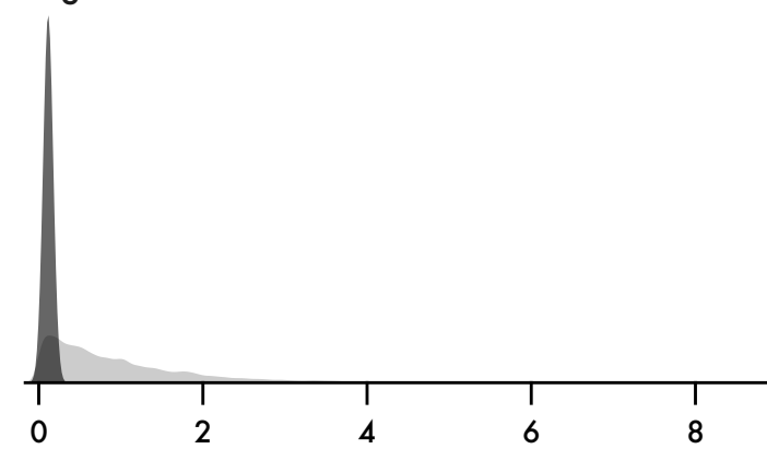
Gamma likelihood
