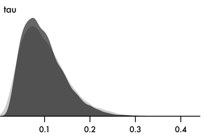
Beta prime likelihood with homogenous variance
