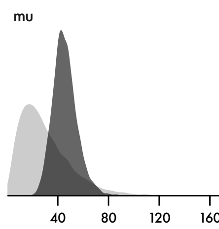
Beta prime likelihood with heterogenous variance
