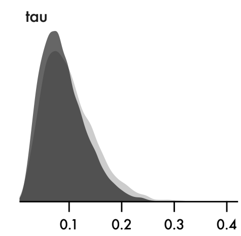
Beta prime likelihood with heterogenous variance
