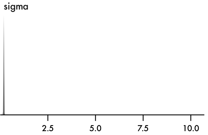
Gamma likelihood
