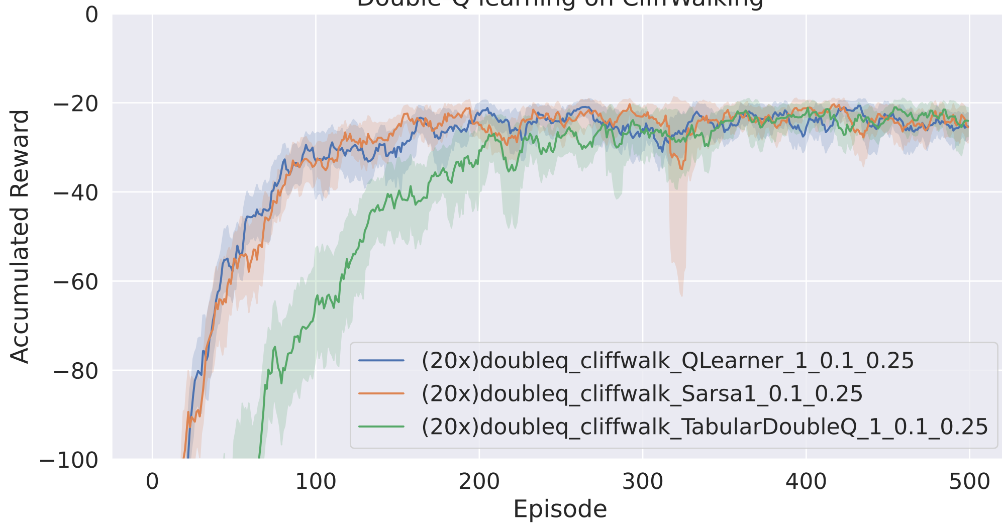
Double-Q learning on CliffWalking
