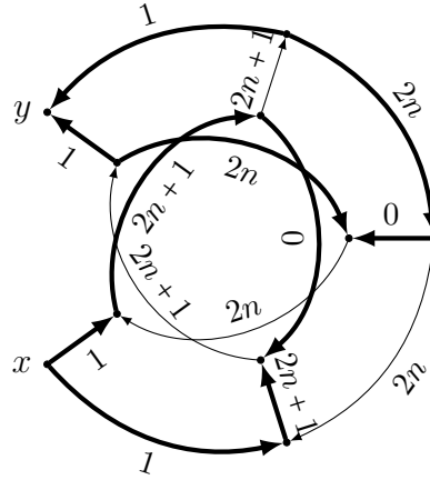
Figure 6.2: (1/(2n)) -flow-pair on Q
