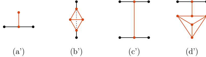
Figure 4.2: Cubic poles extensions
