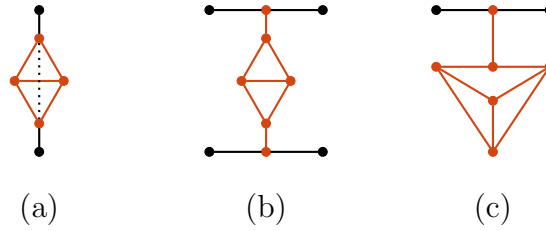
Figure 2.2: Prime graph extensions
