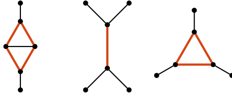
Figure 4.3: Base cases with good edges emphasised
