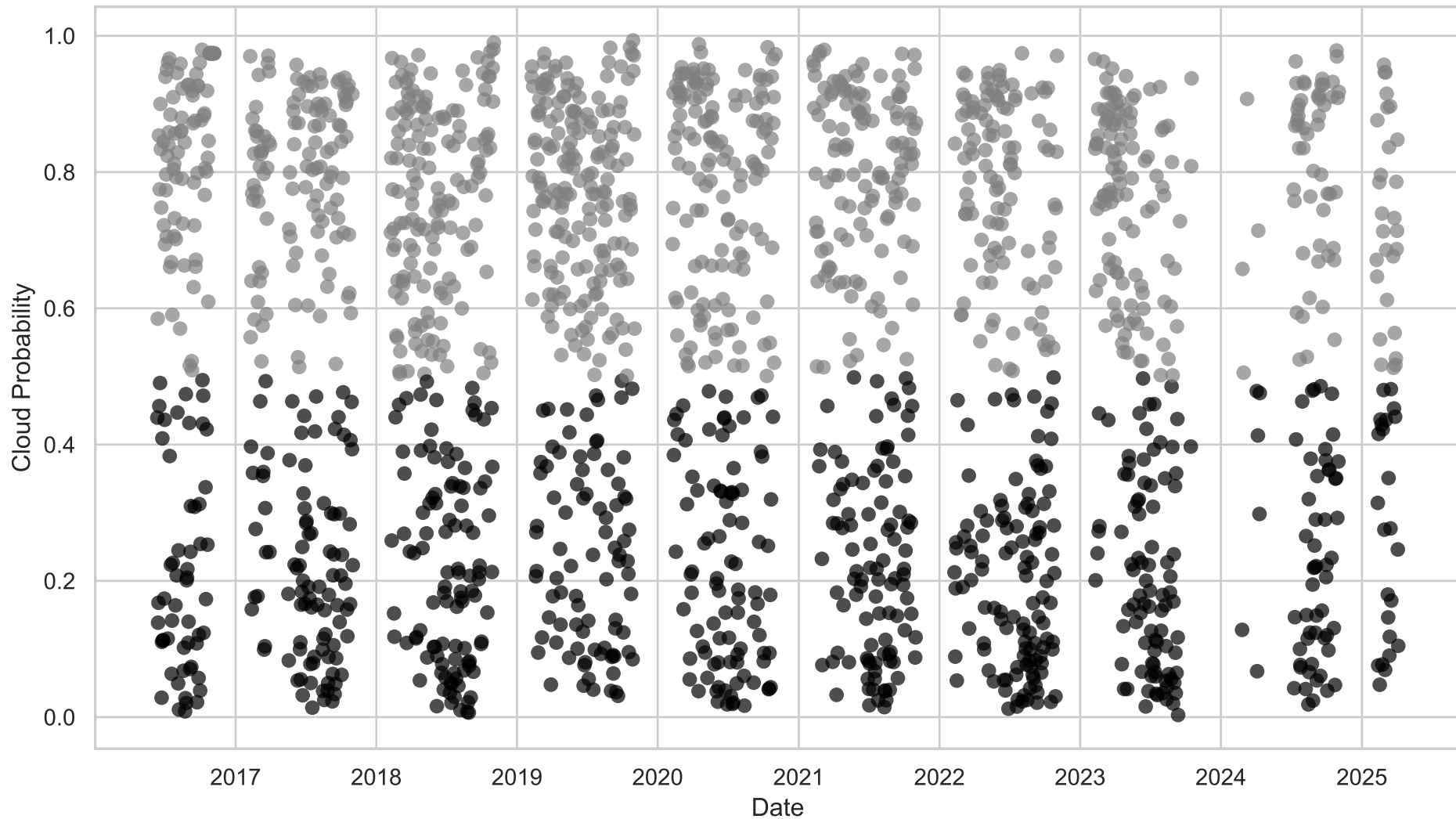
Cloud Probability Over Time
