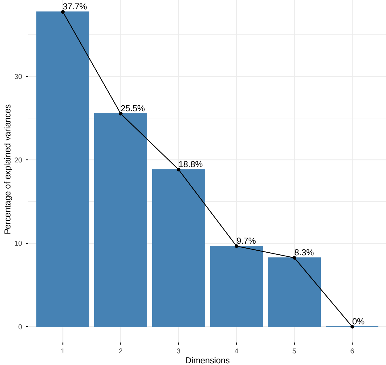
Variance explained by PC
