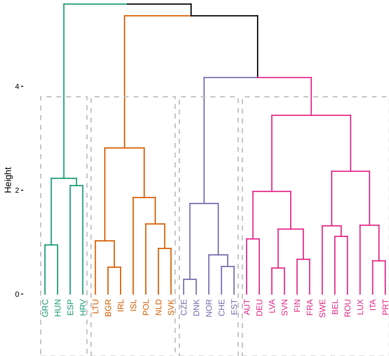
Dendrogram – complete linkage on PC1–PC3
