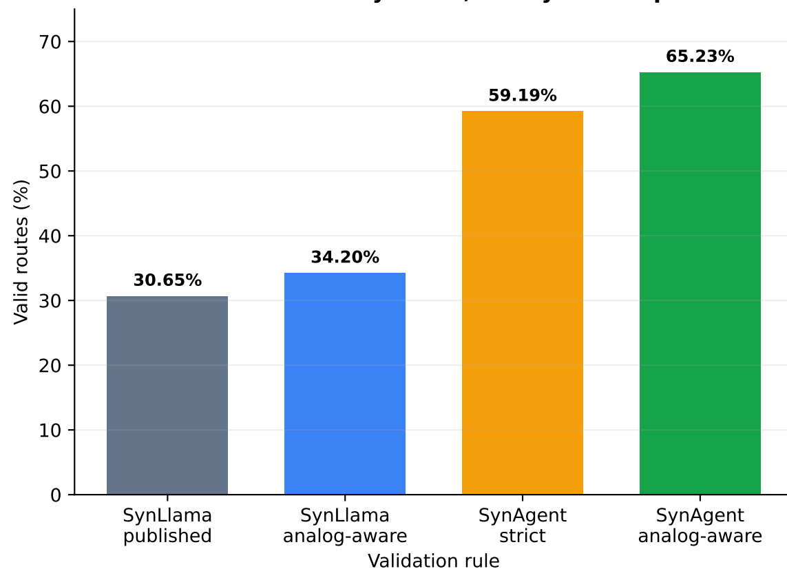
Route-level validity on 10,000 SynLlama paths
