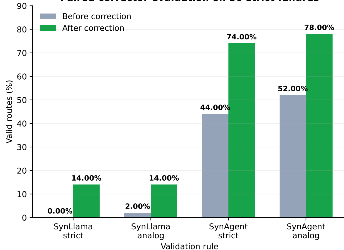
Paired corrector evaluation on 50 strict failures
