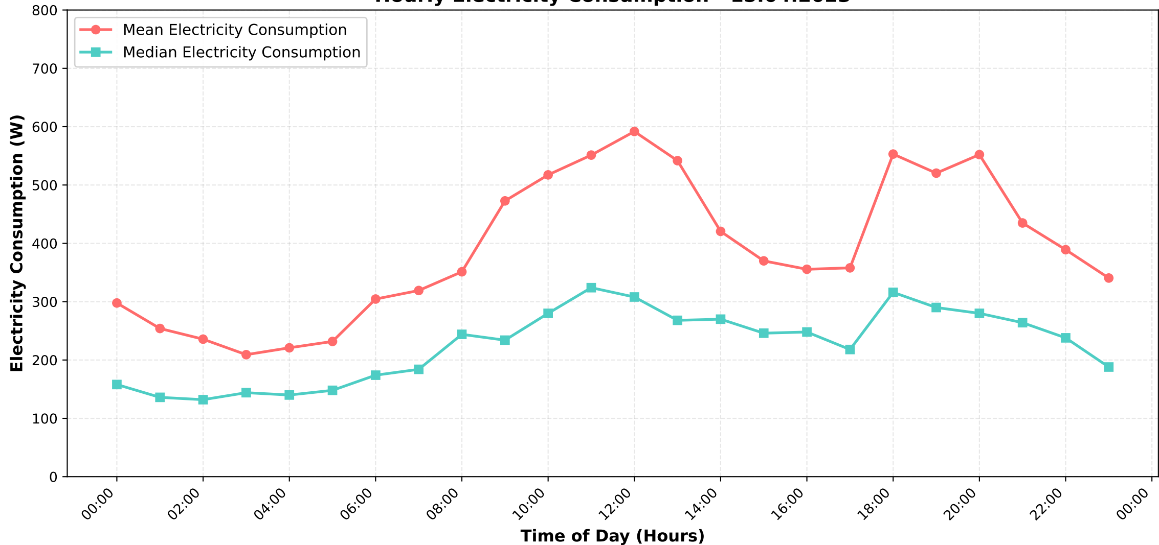
Hourly Electricity Consumption - 15.04.2023
