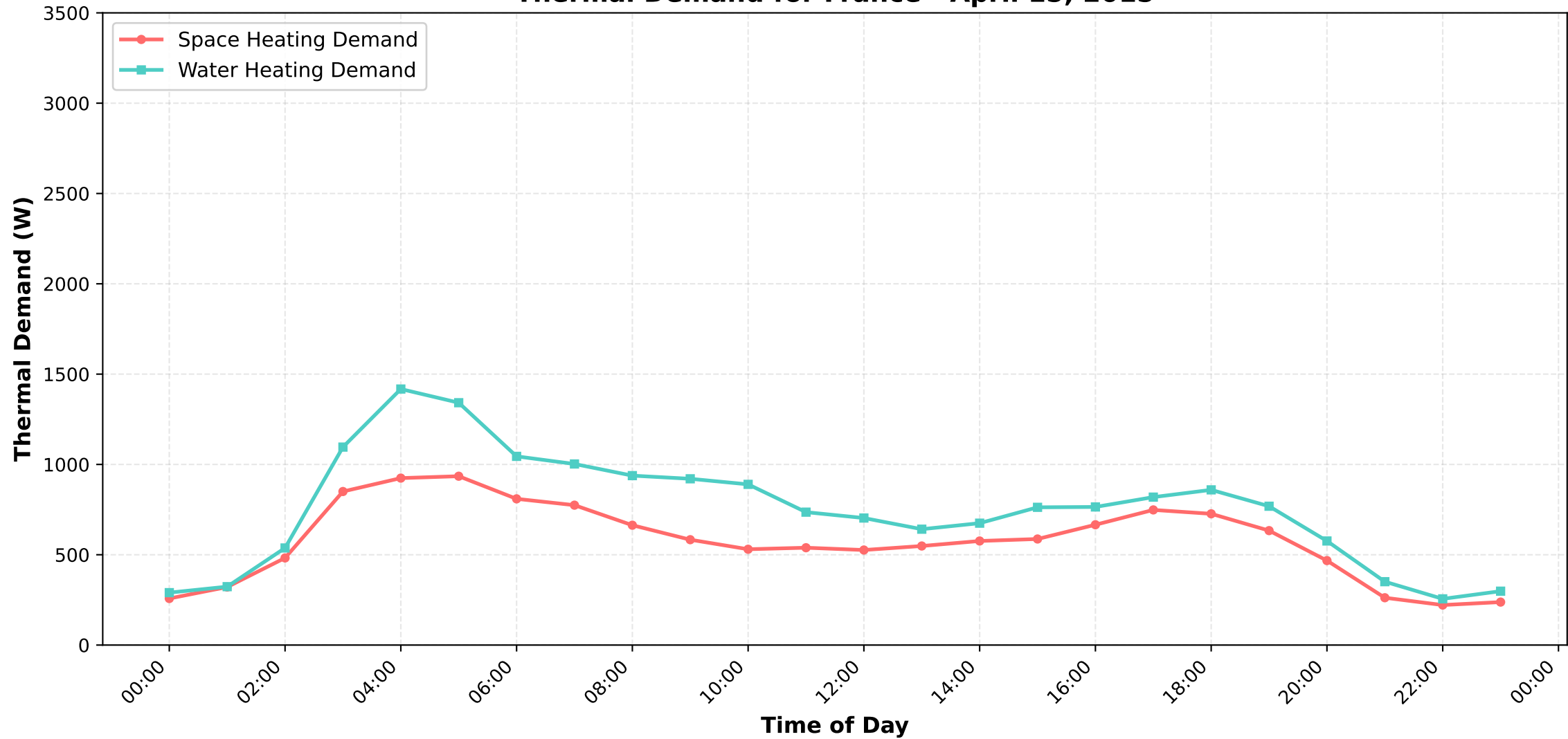
Thermal Demand for France - April 15, 2015
