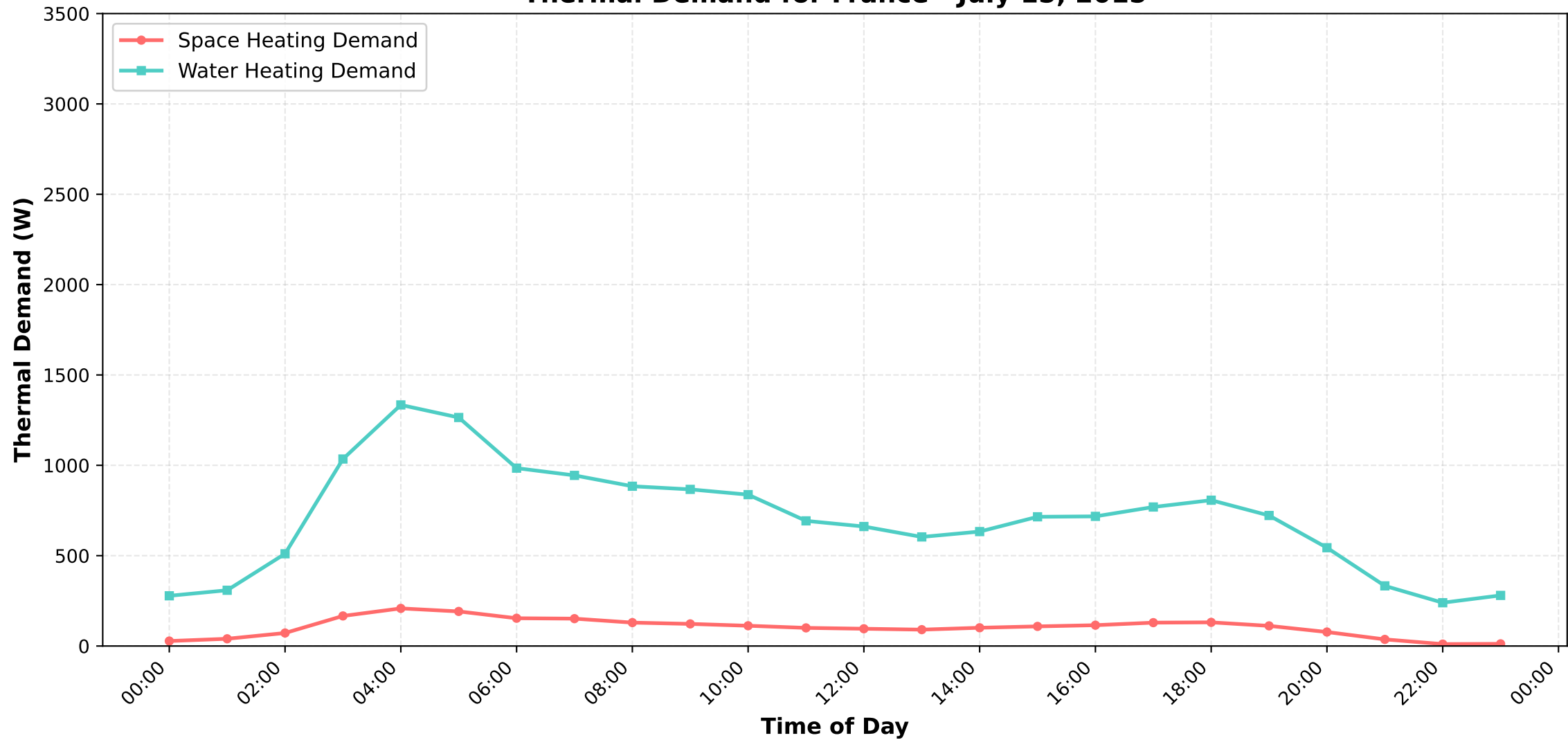
Thermal Demand for France - July 15, 2015
