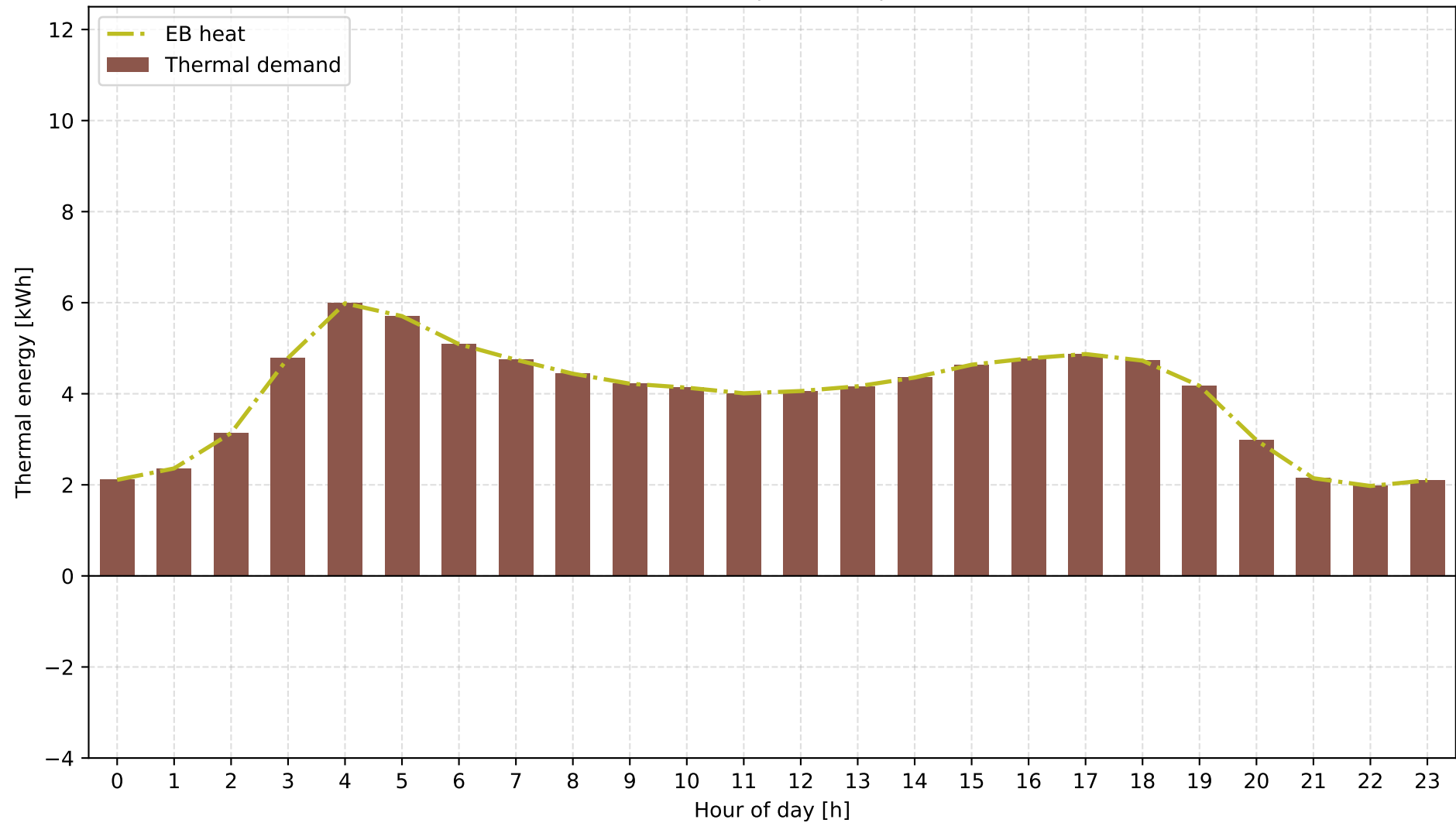
B: Grid + Electric Boiler | Autumn | Thermal Energy
