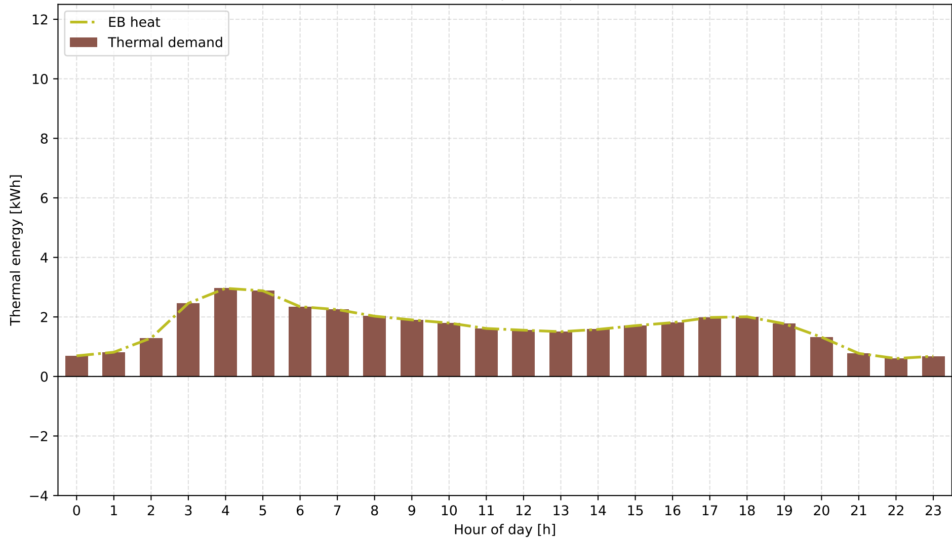
B: Grid + Electric Boiler | Spring | Thermal Energy
