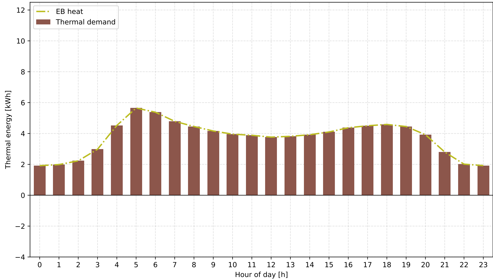
B: Grid + Electric Boiler | Winter | Thermal Energy
