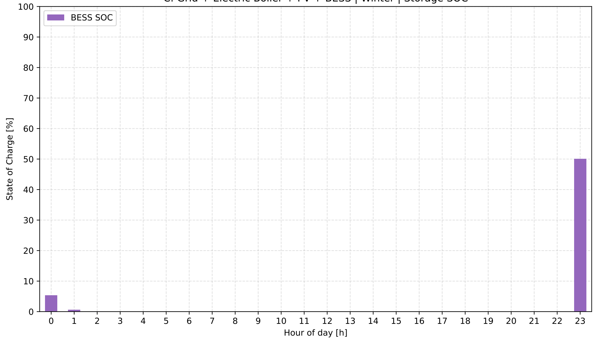
C: Grid + Electric Boiler + PV + BESS | Winter | Storage SOC
