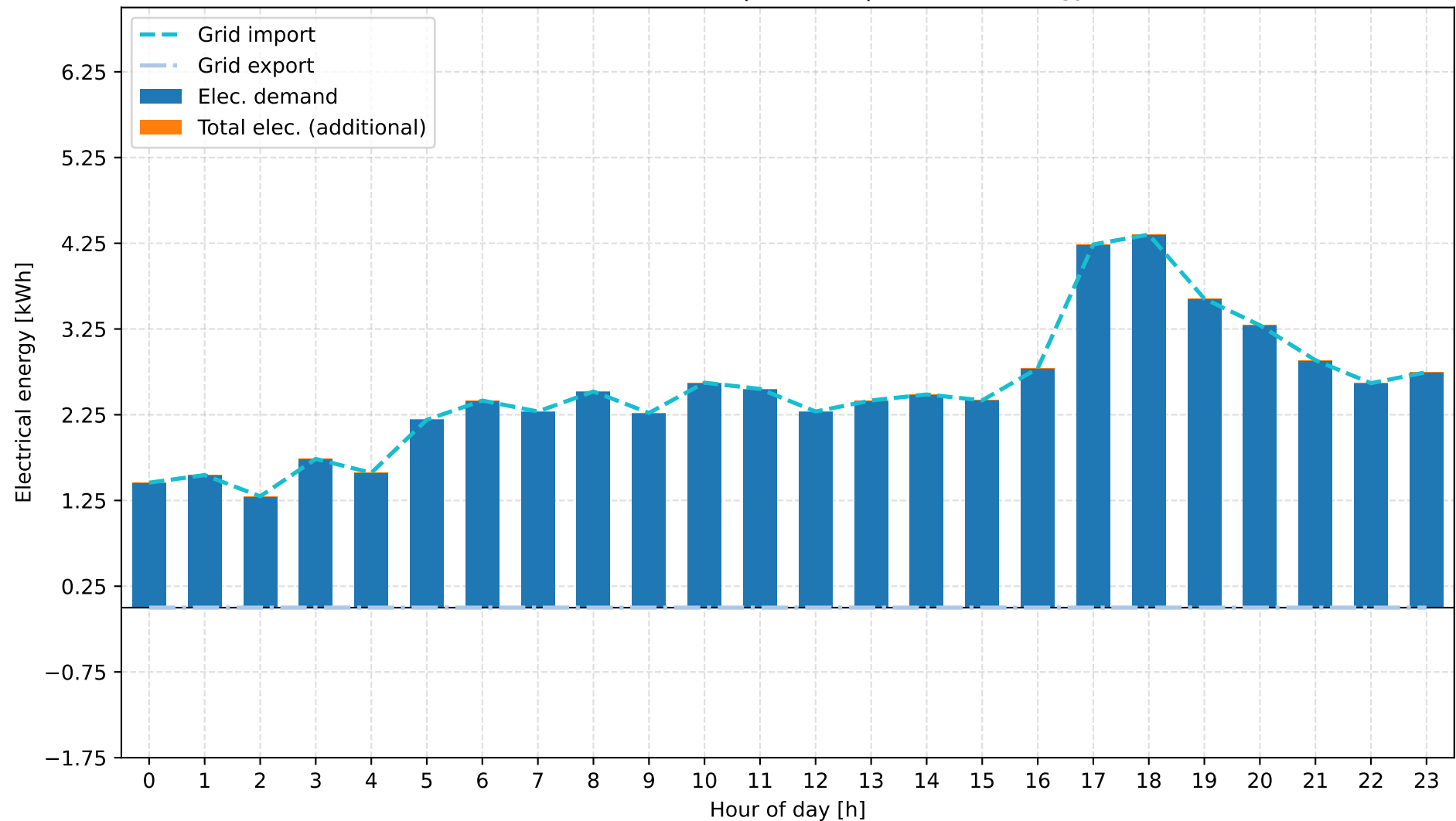
A: Grid + Gas Boiler | Autumn | Electrical Energy
