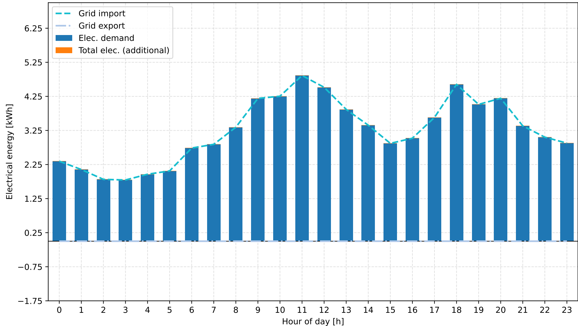
A: Grid + Gas Boiler | Spring | Electrical Energy
