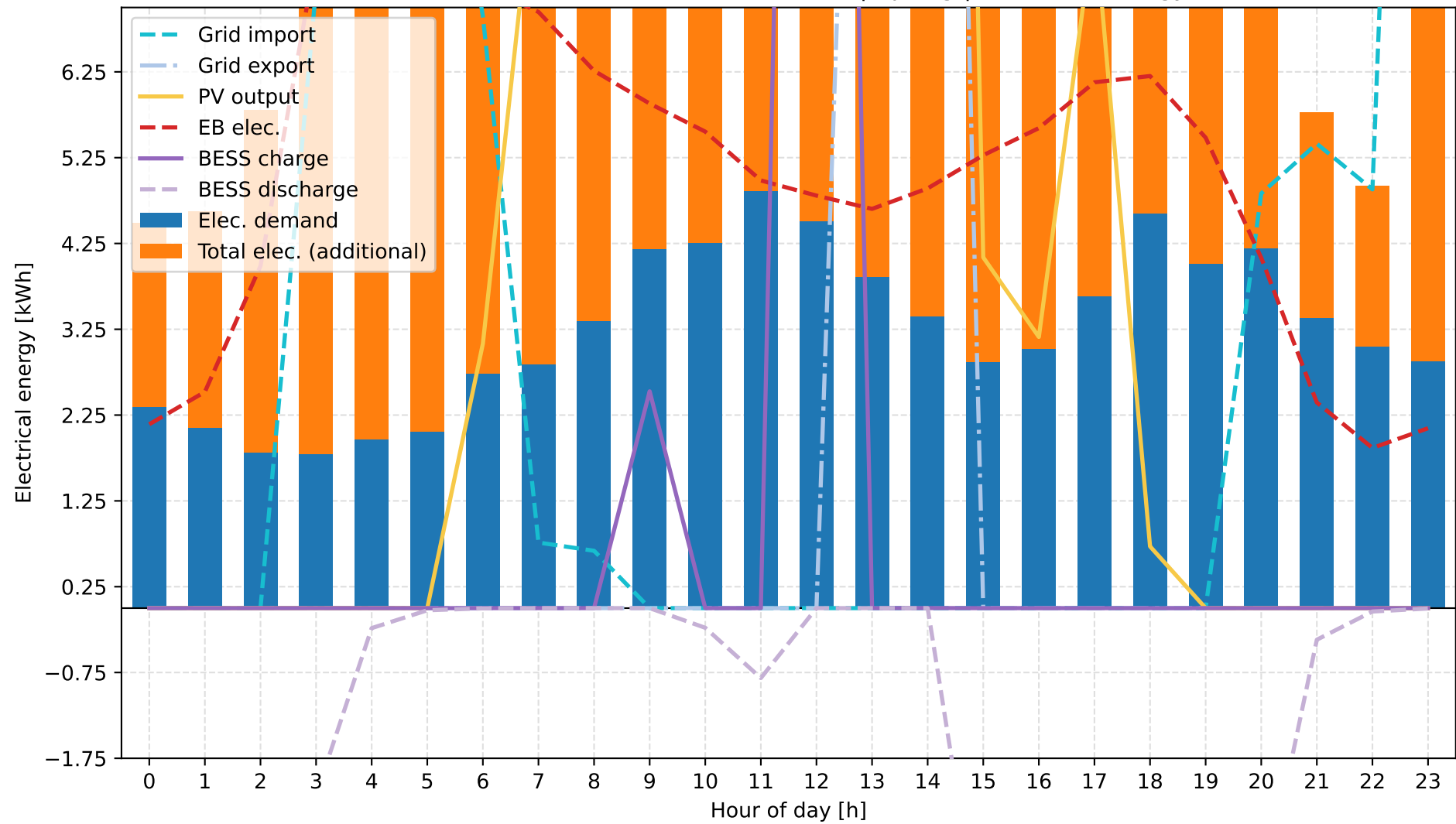
C: Grid + Electric Boiler + PV + BESS | Spring | Electrical Energy
